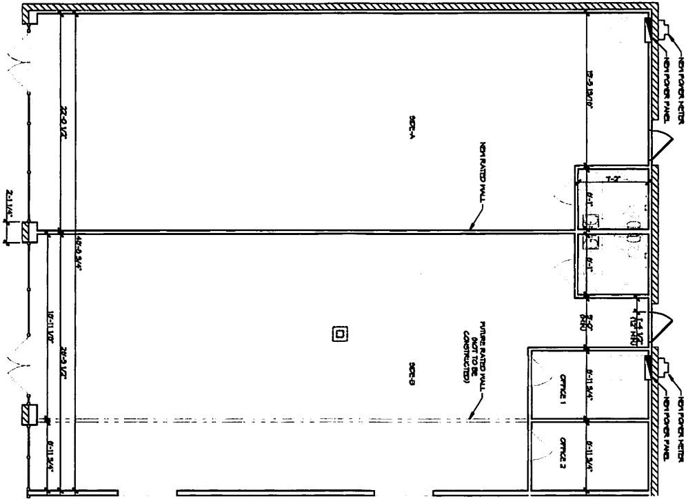
2 FLOOR PLAN
