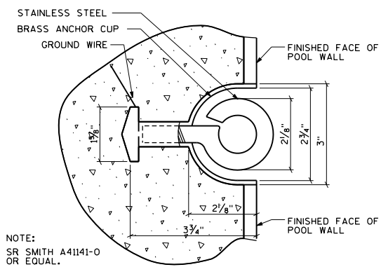
ROPE ANCHOR DETAIL 4 SCALE: NONE
