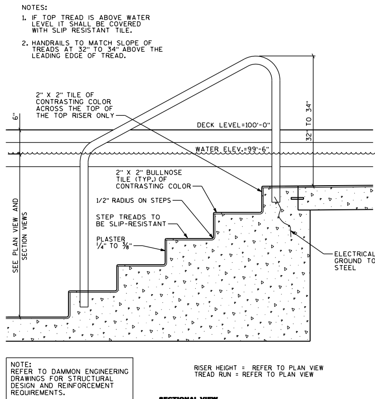
FOUR TREAD STAIR DETAIL 5 SCALE: NONE
