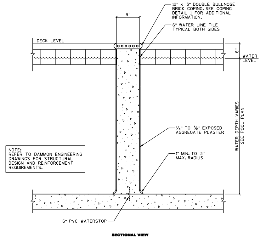
TYPICAL COMMON WALL DETAIL 3 SCALE: 1" = 1'
