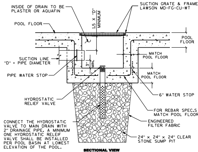
MAIN DRAIN DETAIL 18" X 36" 2 SCALE: 1" = 1'
