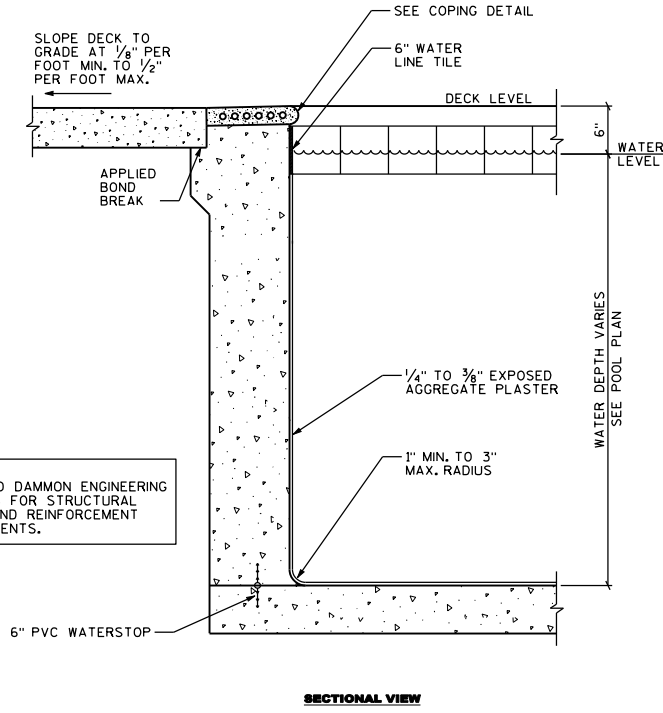
TYPICAL POOL WALL DETAIL 2 SCALE: 1" = 1'
