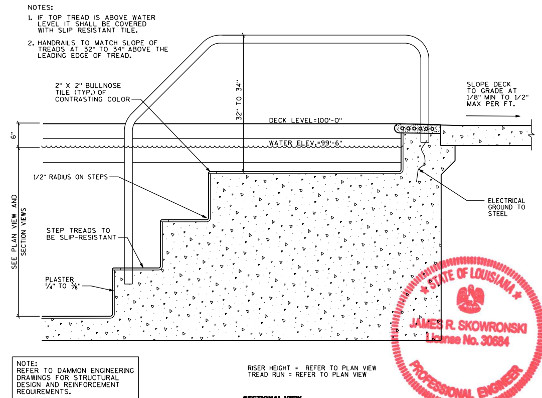
THREE TREAD STAIR DETAIL 6 SCALE: NONE
