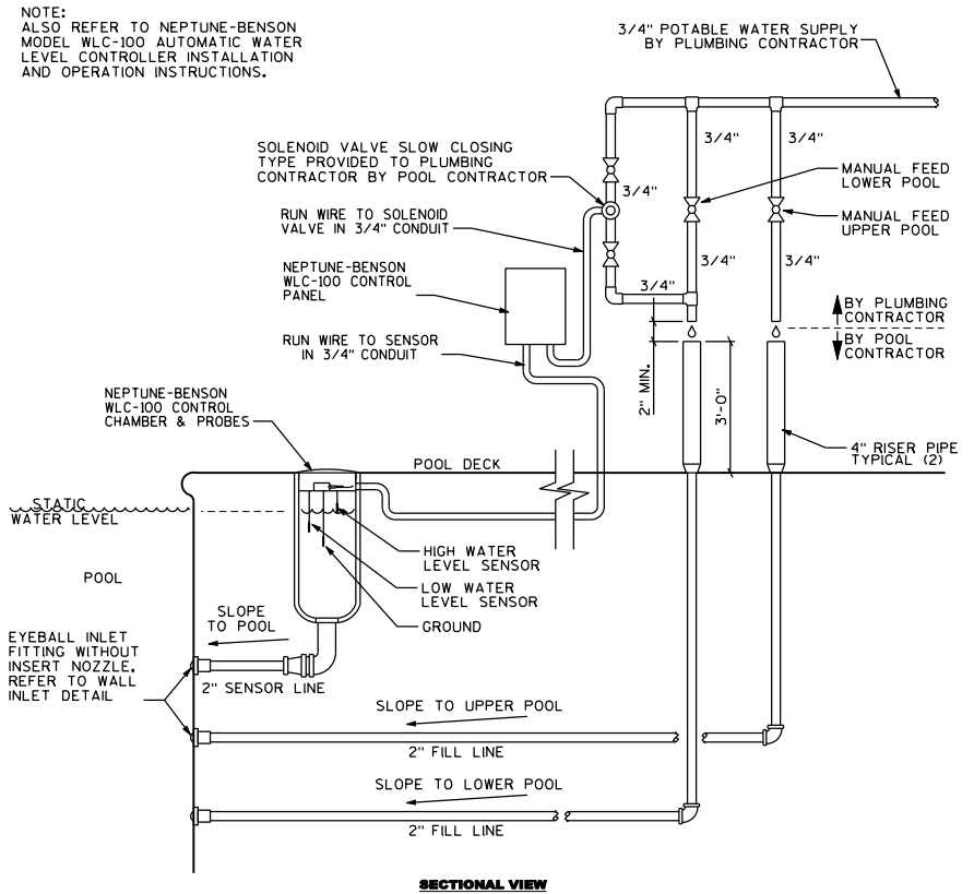
AUTO-FILL AND SENSOR DETAIL 3 SCALE: NONE
