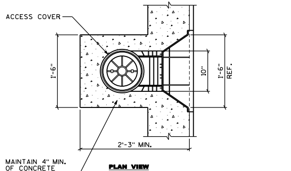
MAIN DRAIN DETAIL 18" X 36" 2 SCALE: 1" = 1'
