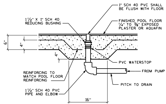
GEYSER DETAIL 3 SCALE: NONE
