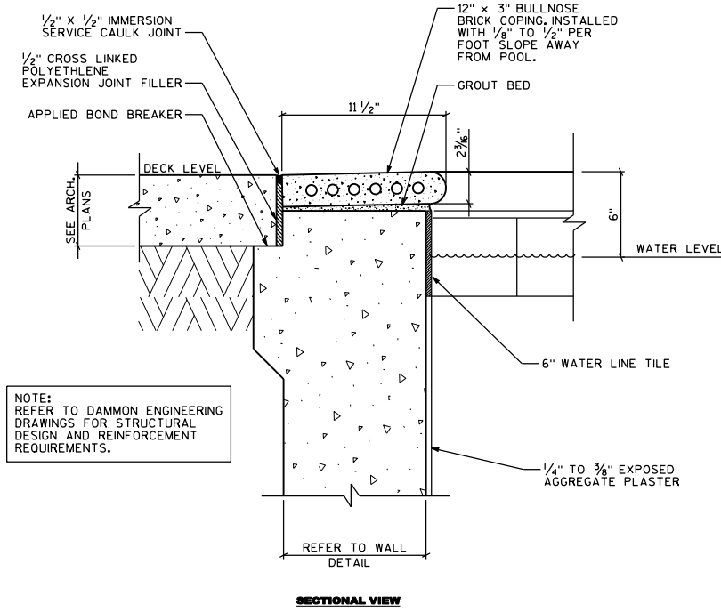
BRICK COPING DETAIL 1 SCALE: NONE
