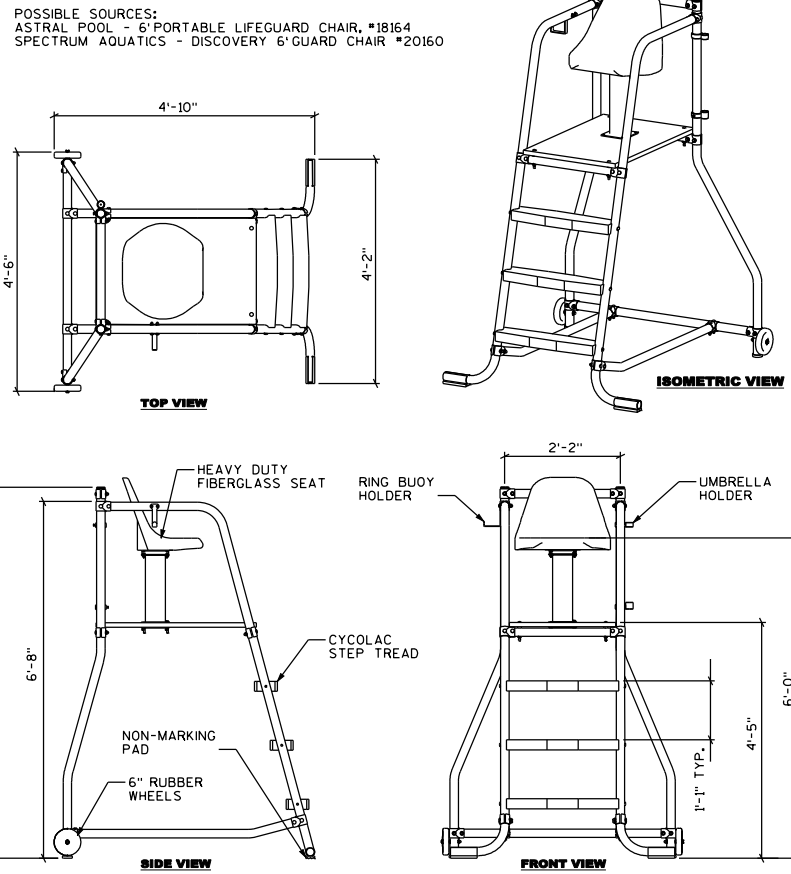
LIFEGUARD STAND DETAIL 2 SCALE: NONE
