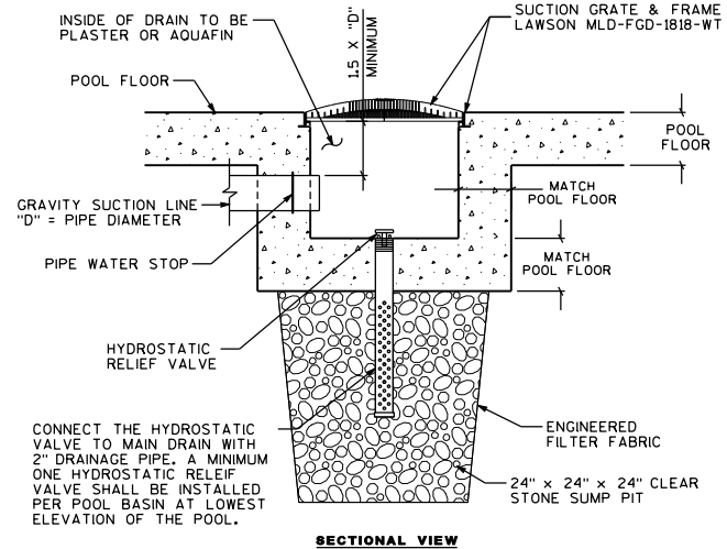
MAIN DRAIN DETAIL 18" X 18" 1 SCALE: 1" = 1'
