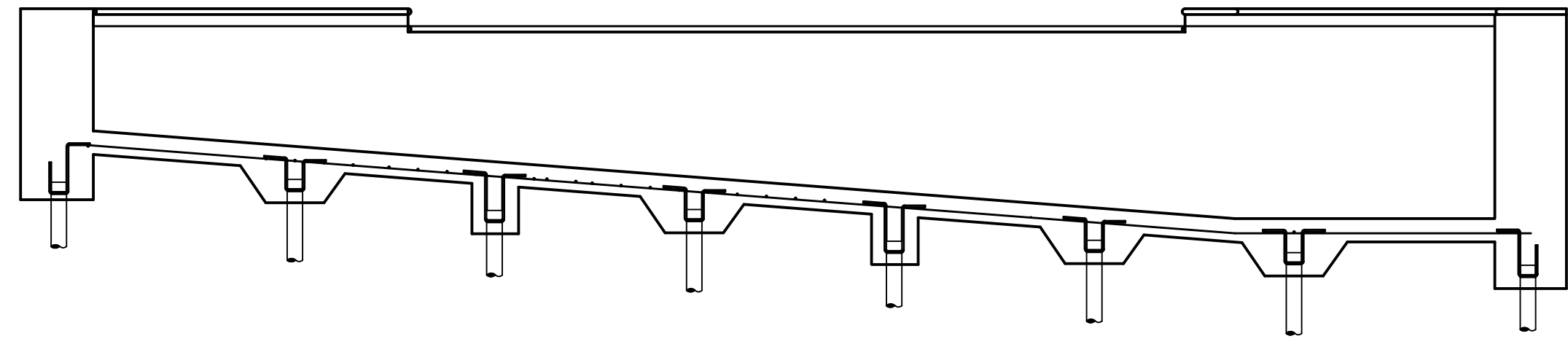
A POOL DETAIL SCALE: 1/4" = 1'-0"
