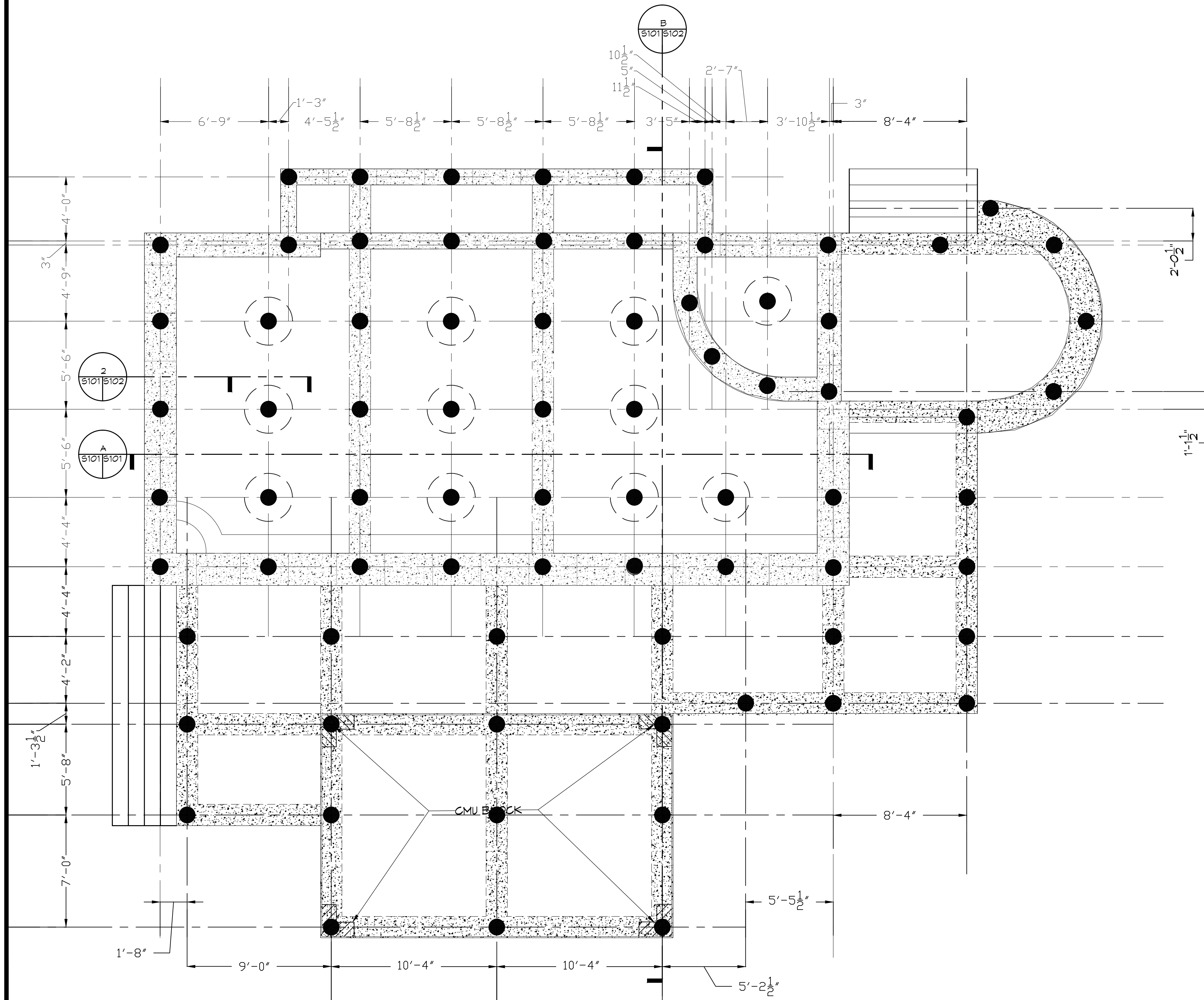
1 POOL & DECK PILING PLAN SCALE: 1/4" = 1'-0"
