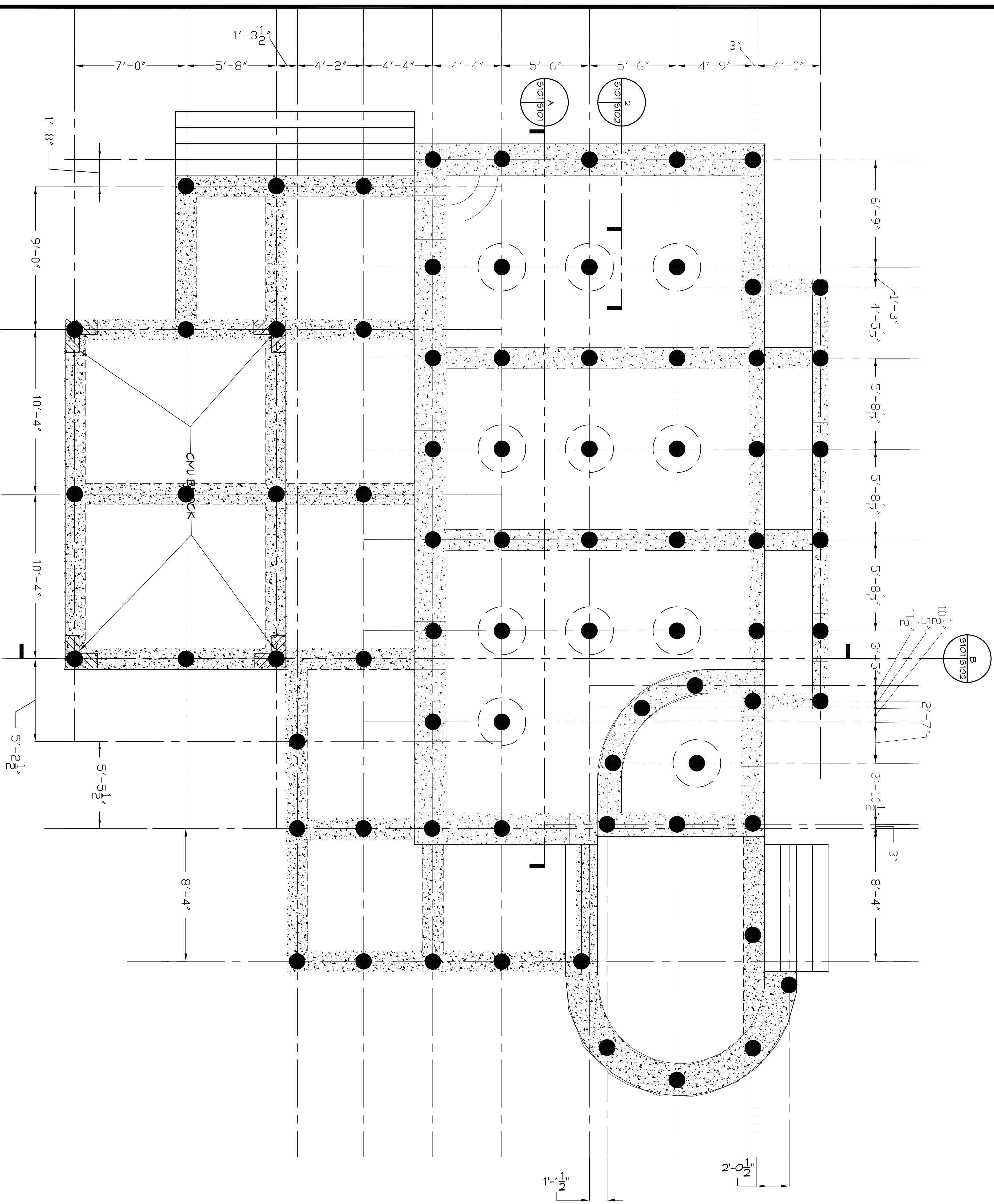
A POOL DETAIL SCALE: 1/4" = 1'-0"
