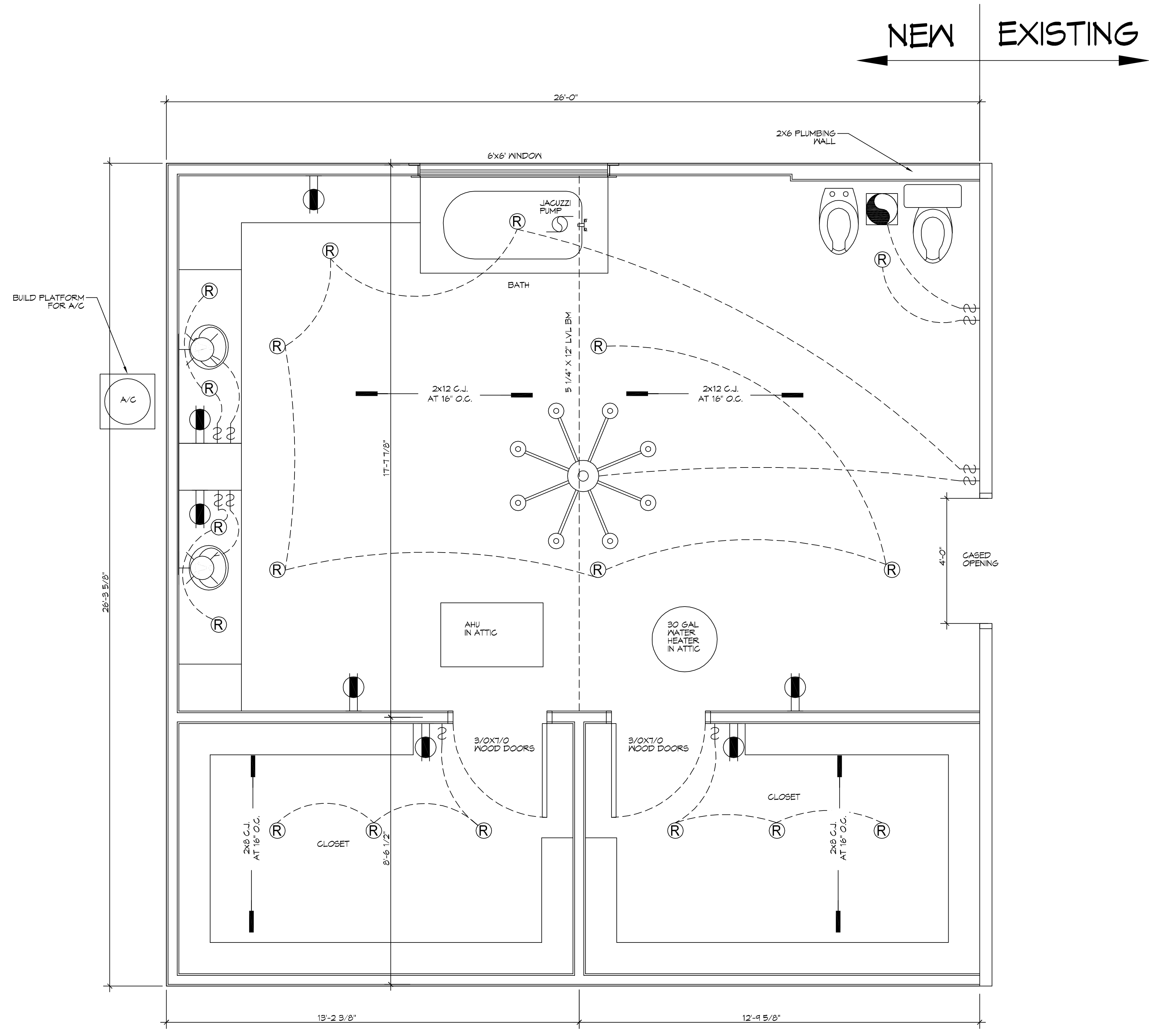
1 BATHROOM LAYOUT SCALE: 1/2" = 1'-0" ARCHITURAL
