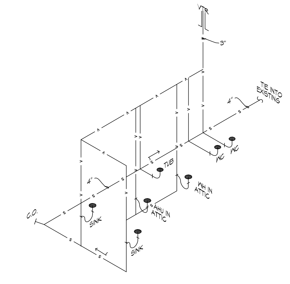
2 PLUMBING LAYOUT SCALE: 1/4" = 1'-0" PLUMBING
