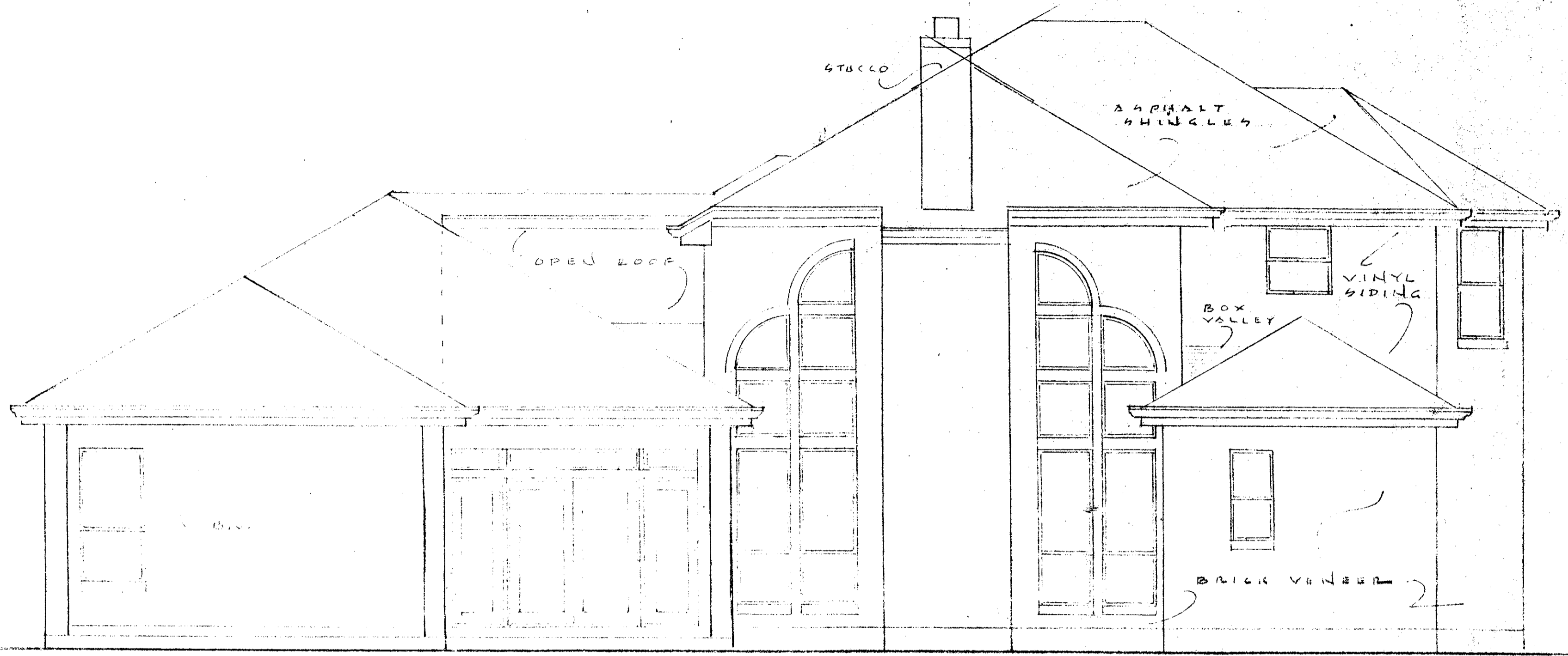
REAR ELEV.
