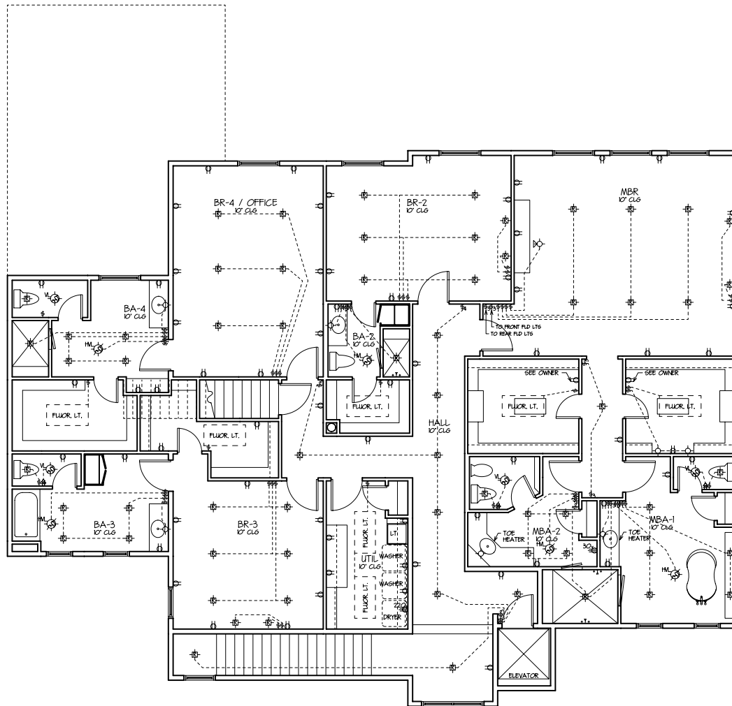
2ND LEVEL ELECTRICAL PLAN SCALE 1/4"=1'-0"
