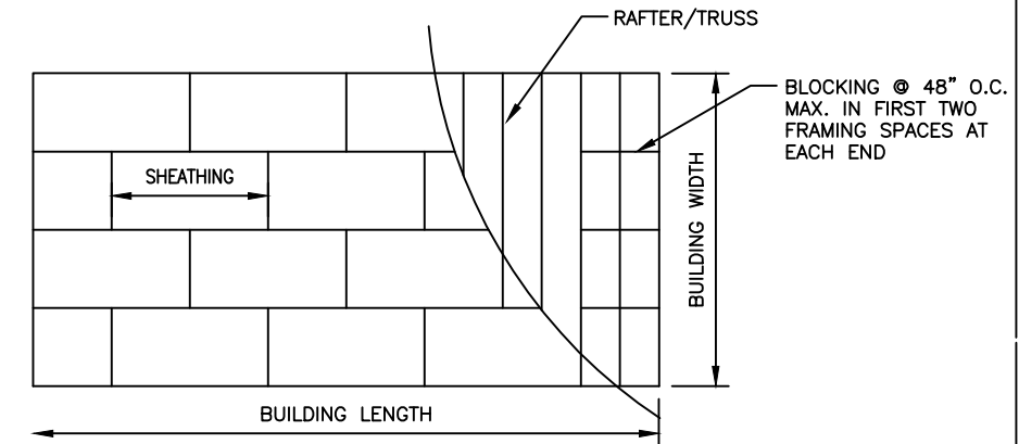
ROOF SHEATHING LAYOUT & ENDWALL ROOF BRACING
