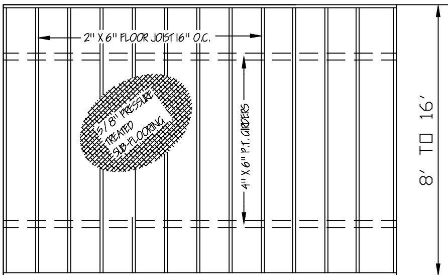
FLOOR FRAMING
