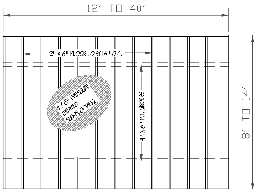
FLOOR FRAMING
