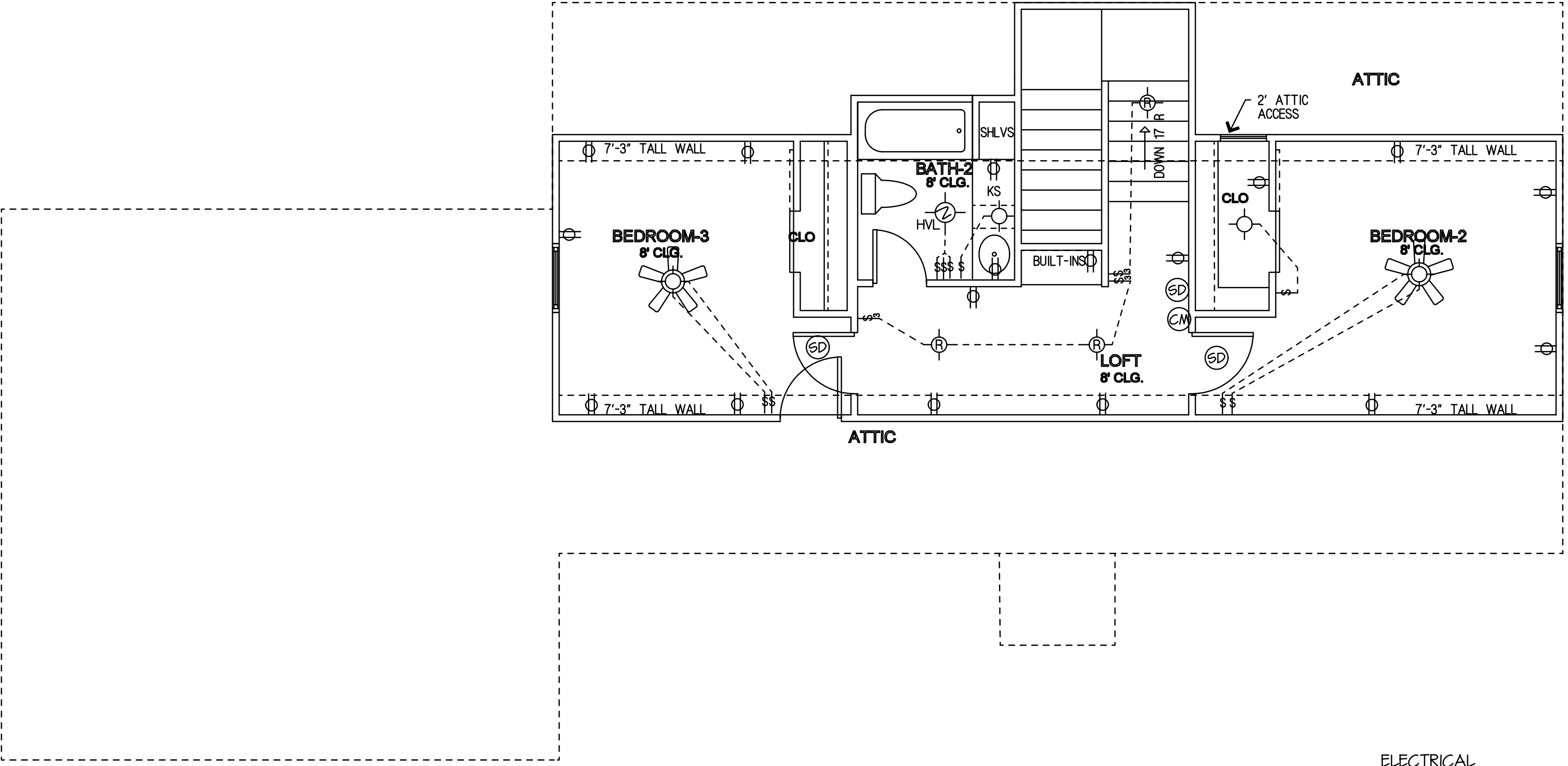
ELECTRICAL SECOND FLOOR PLAN SCALE 1/4" = 1'-0"
