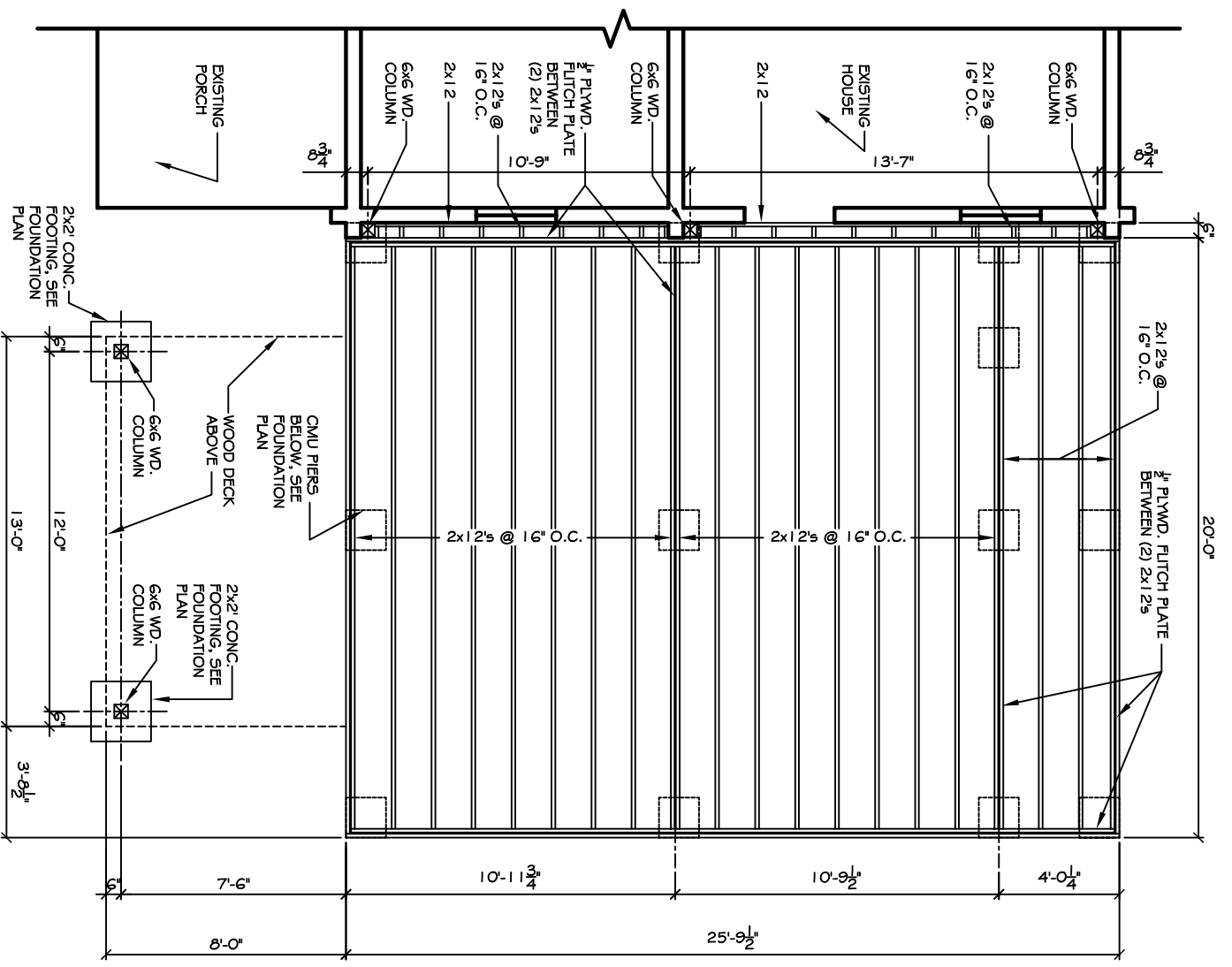
FIRST FLOOR FRAMING PLAN SCALE: 3/8" = 1'
