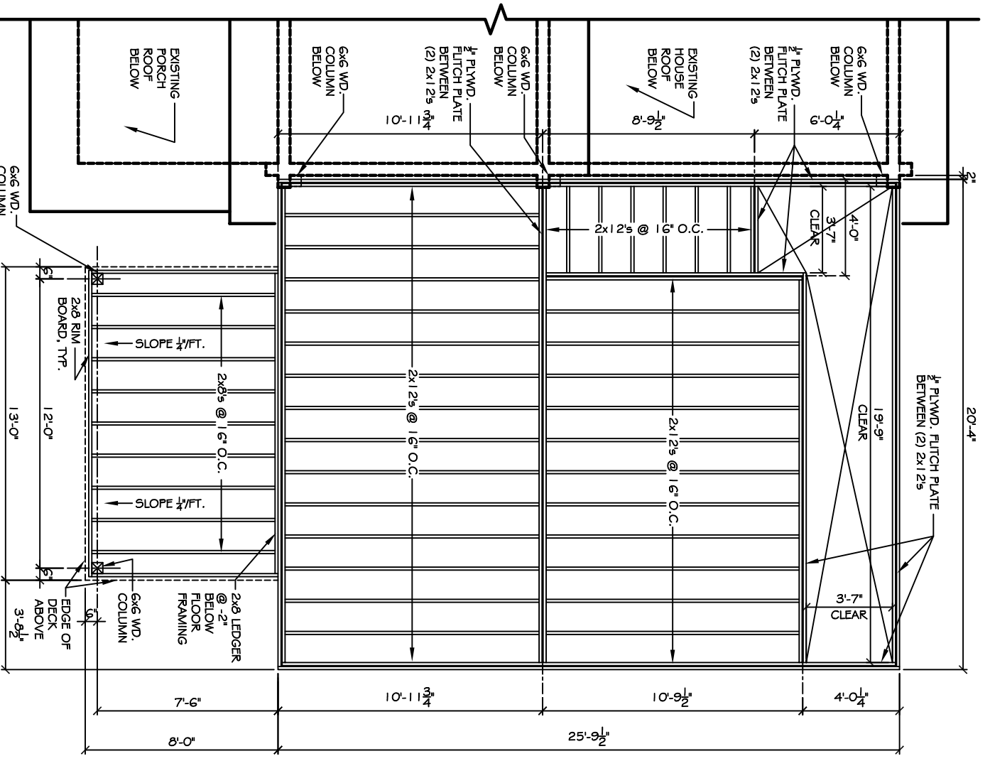
SECOND FLOOR FRAMING PLAN SCALE: 3/8" = 1'
