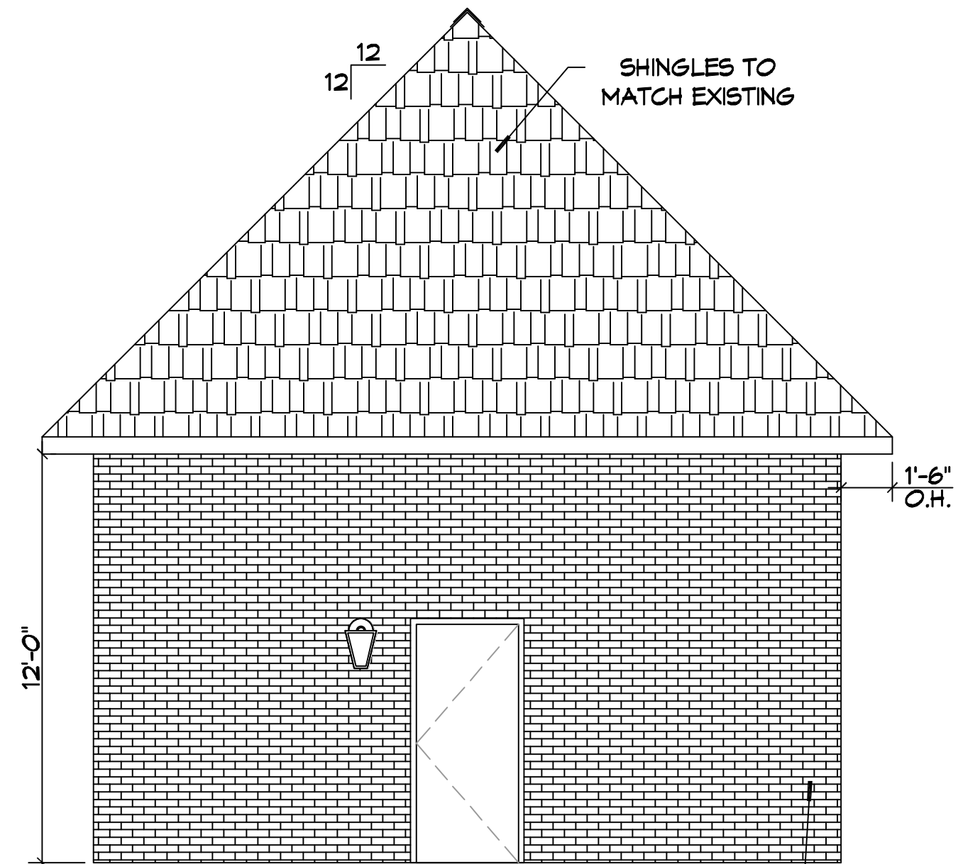
5 REAR ELEVATION SCALE: 1/4"=1'-0"
