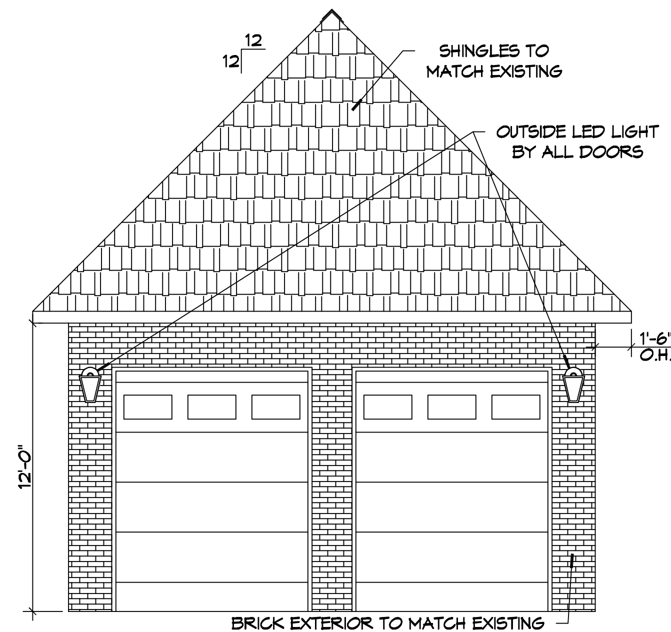
3 FRONT ELEVATION SCALE: 1/4"=1'-0"
