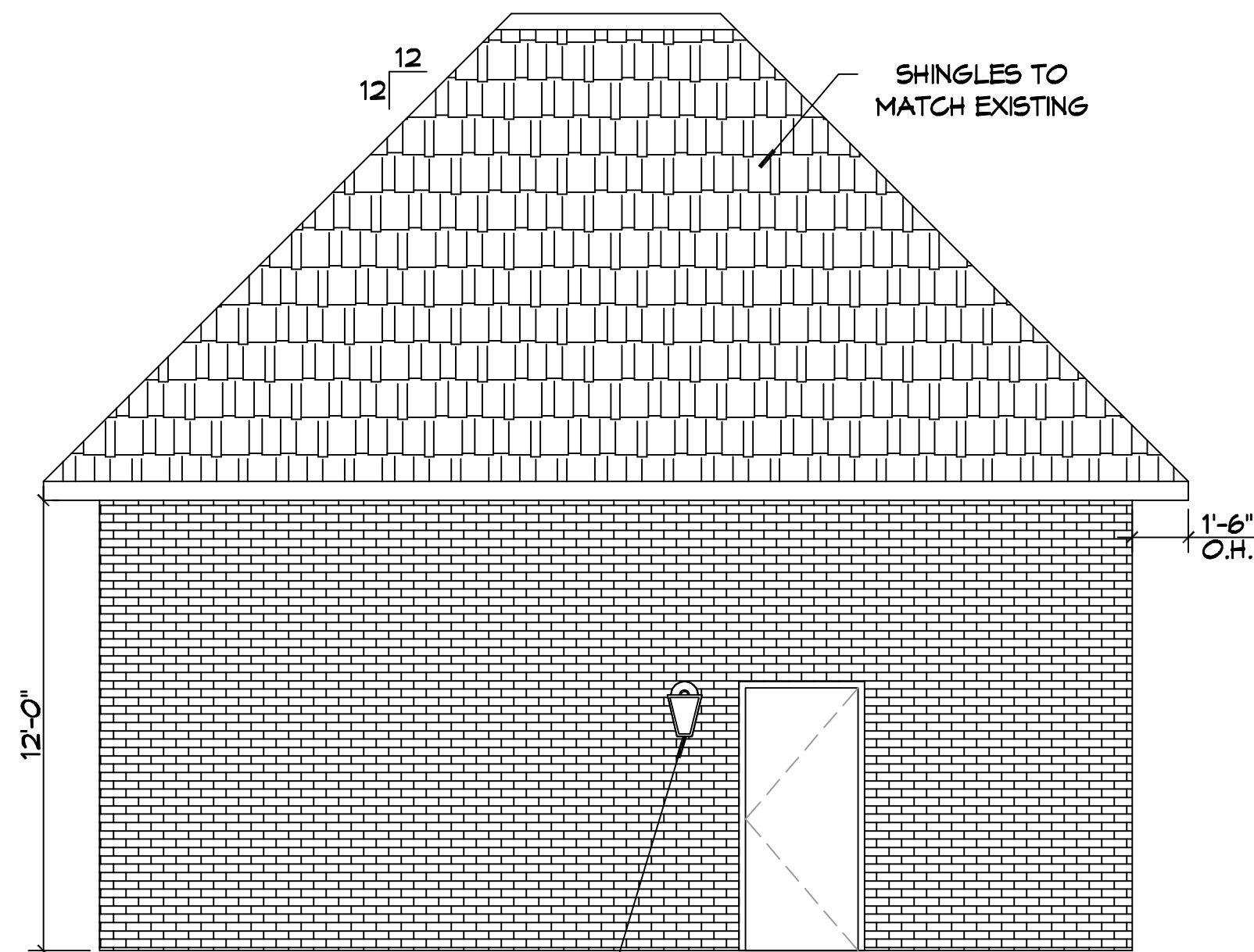
6 RIGHT ELEVATION SCALE: 1/4"=1'-0"
