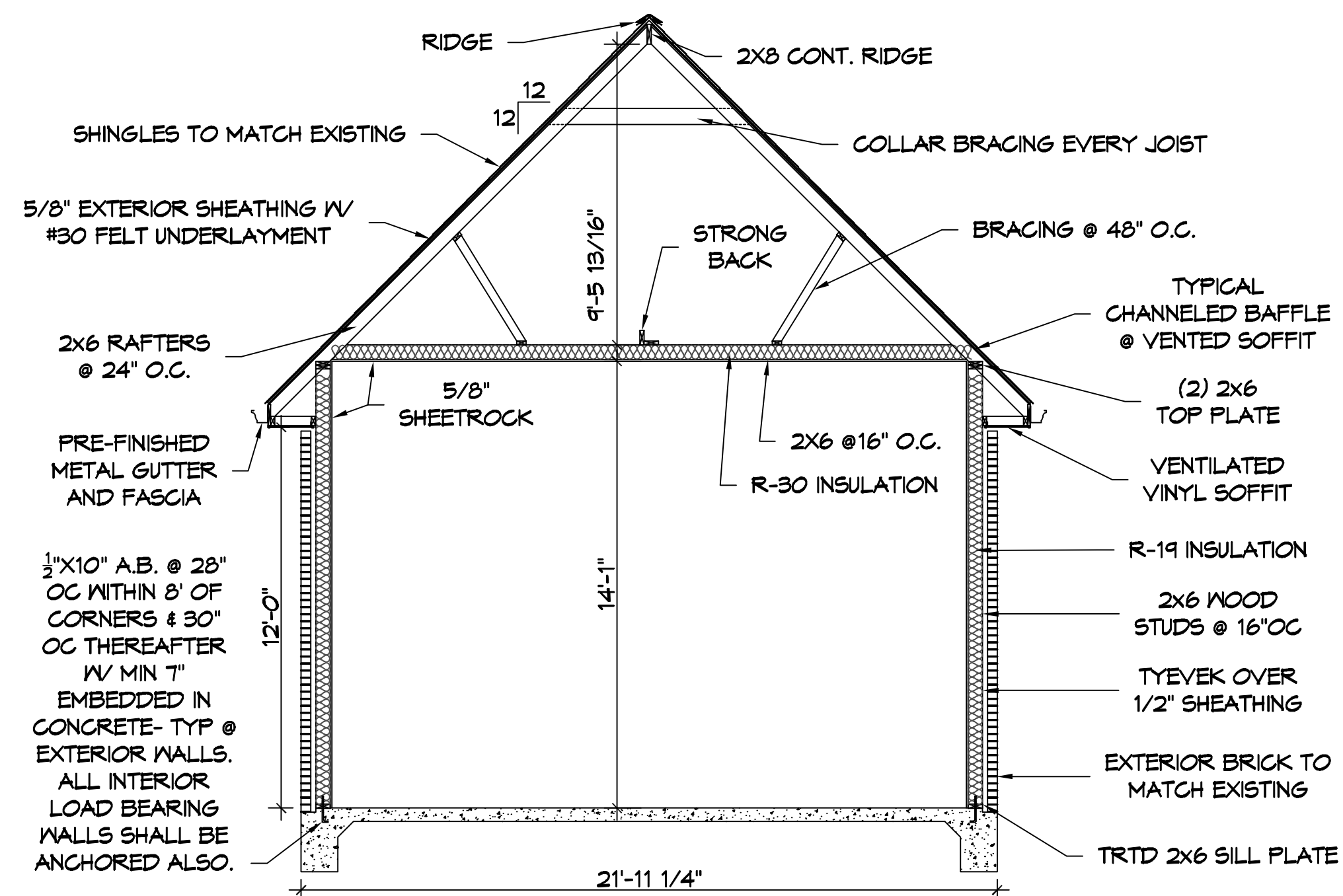
7 SECTION VIEW SCALE: 1/4"=1'-0"
