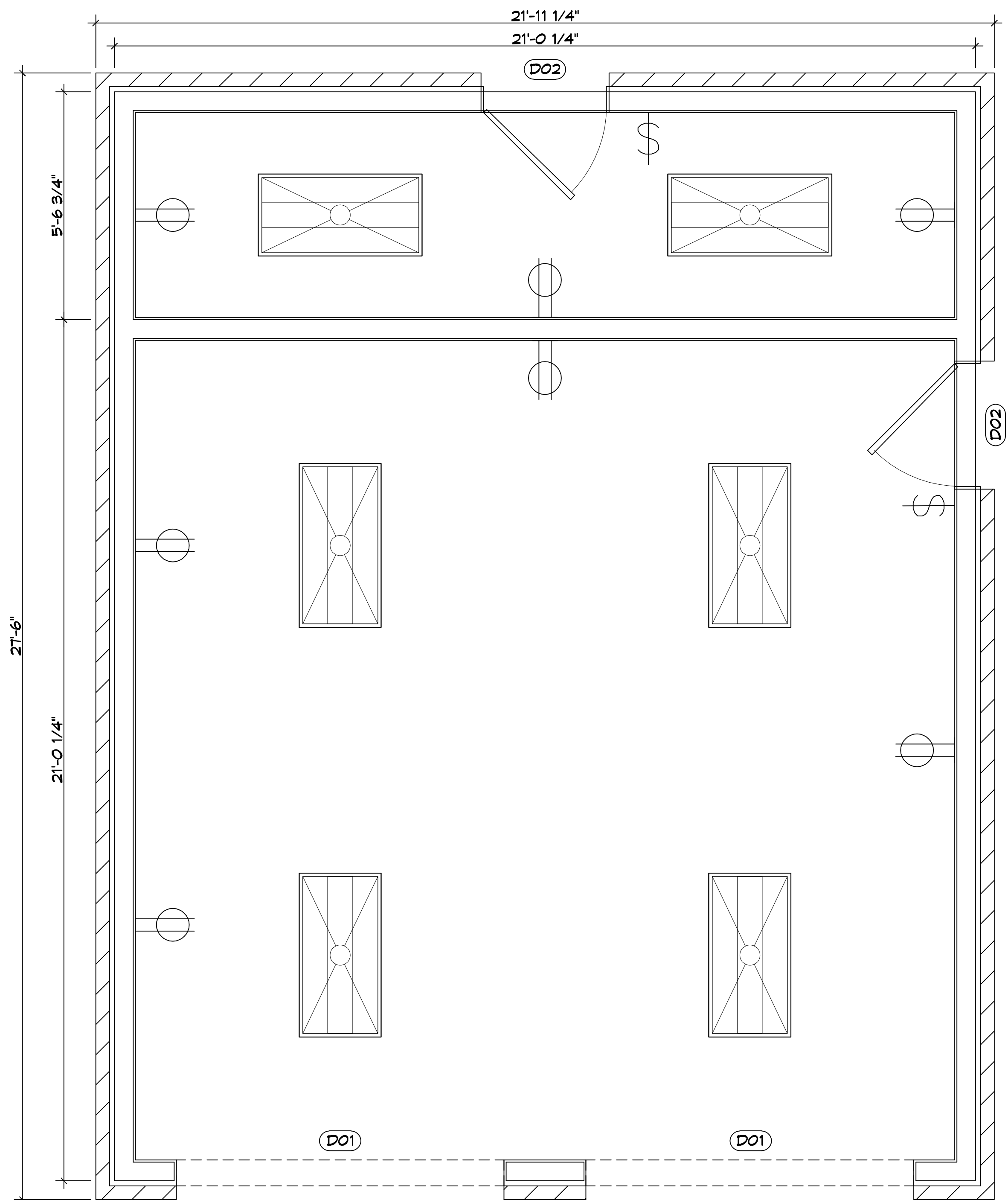
2 FLOOR PLAN SCALE: 1/2"=1'-0"
