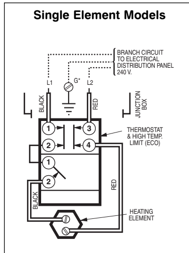
Wiring Diagrams for Type-59T Therm-o-disc Thermostats
