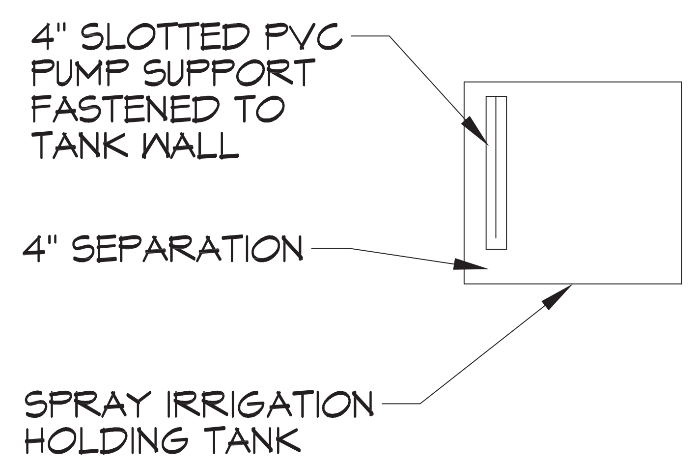
SPRAY IRRIGATION HOLDING TANK PUMP SUPPORT SCALE: 1" = 20'-0"
