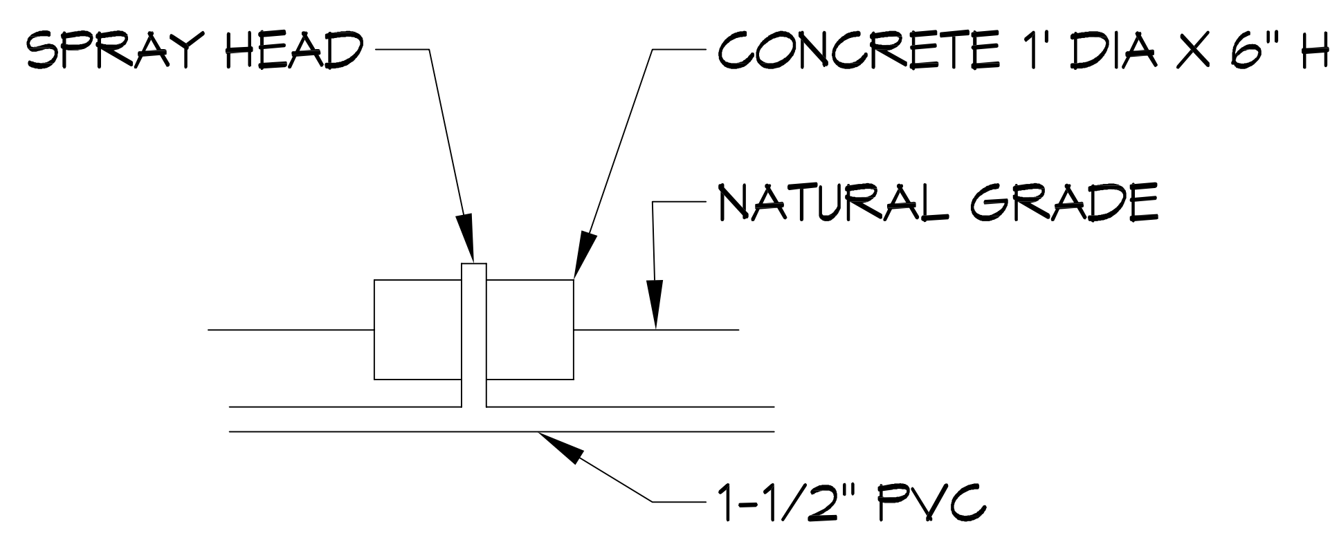
SPRAY HEAD SUPPORT DETAIL SCALE: 1" = 20'-0"
