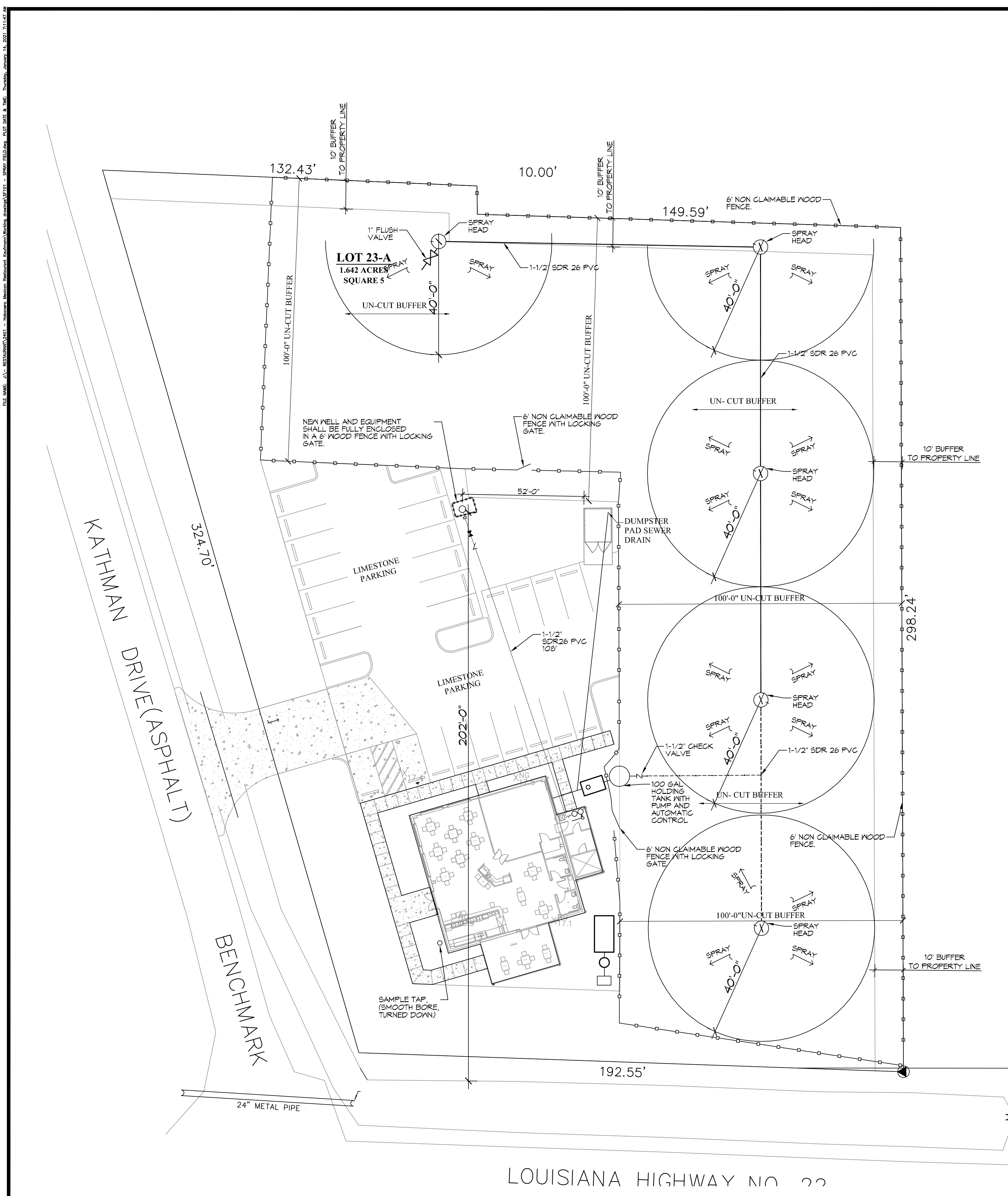
SPRAY IRRIGATION FIELD (5 SPRAY HEADS) SITE PLAN SCALE: 1" = 20'-0"
