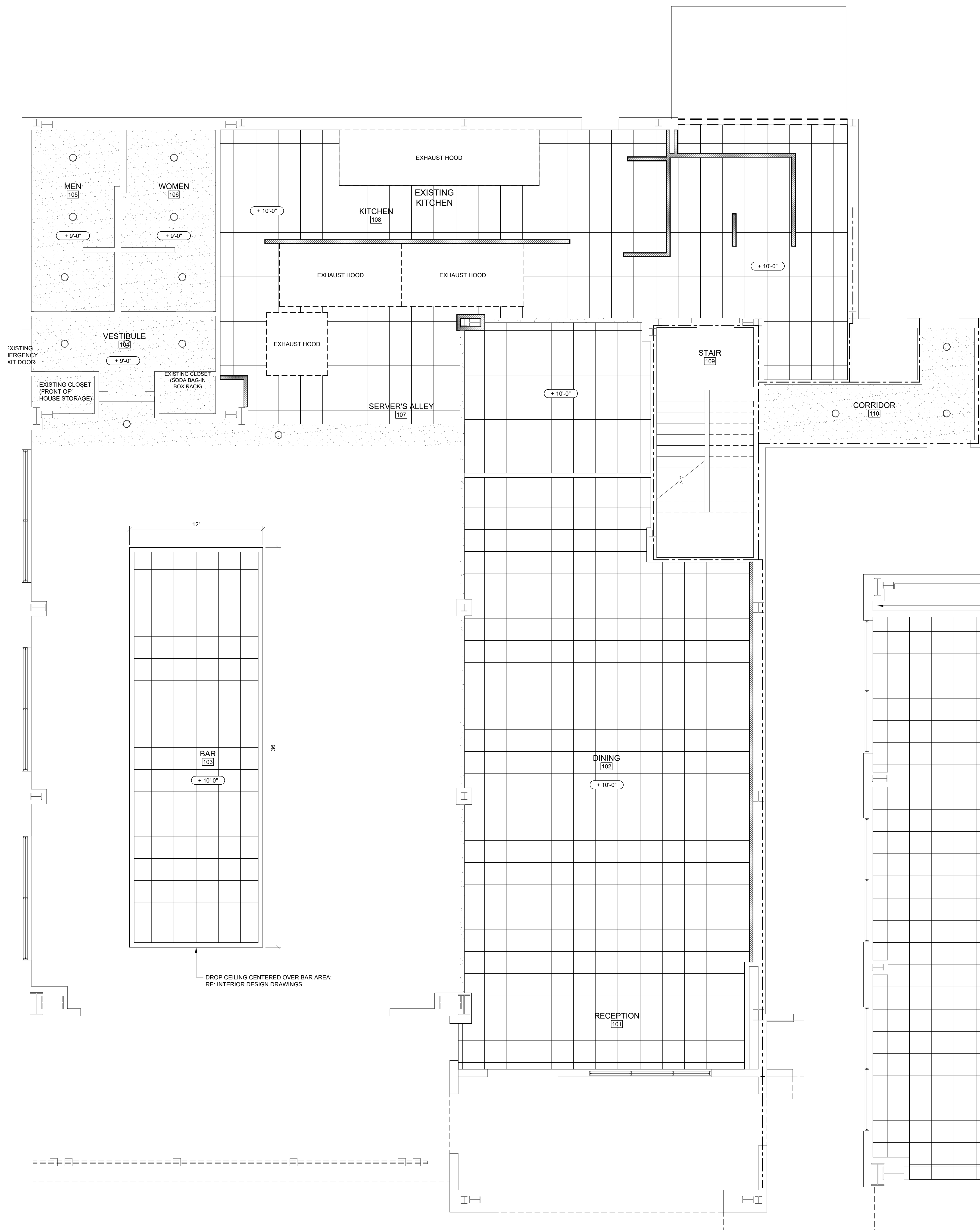
1 REFLECTED CEILING PLAN - FIRST FLOOR SCALE: 1/4" = 1'-0"
