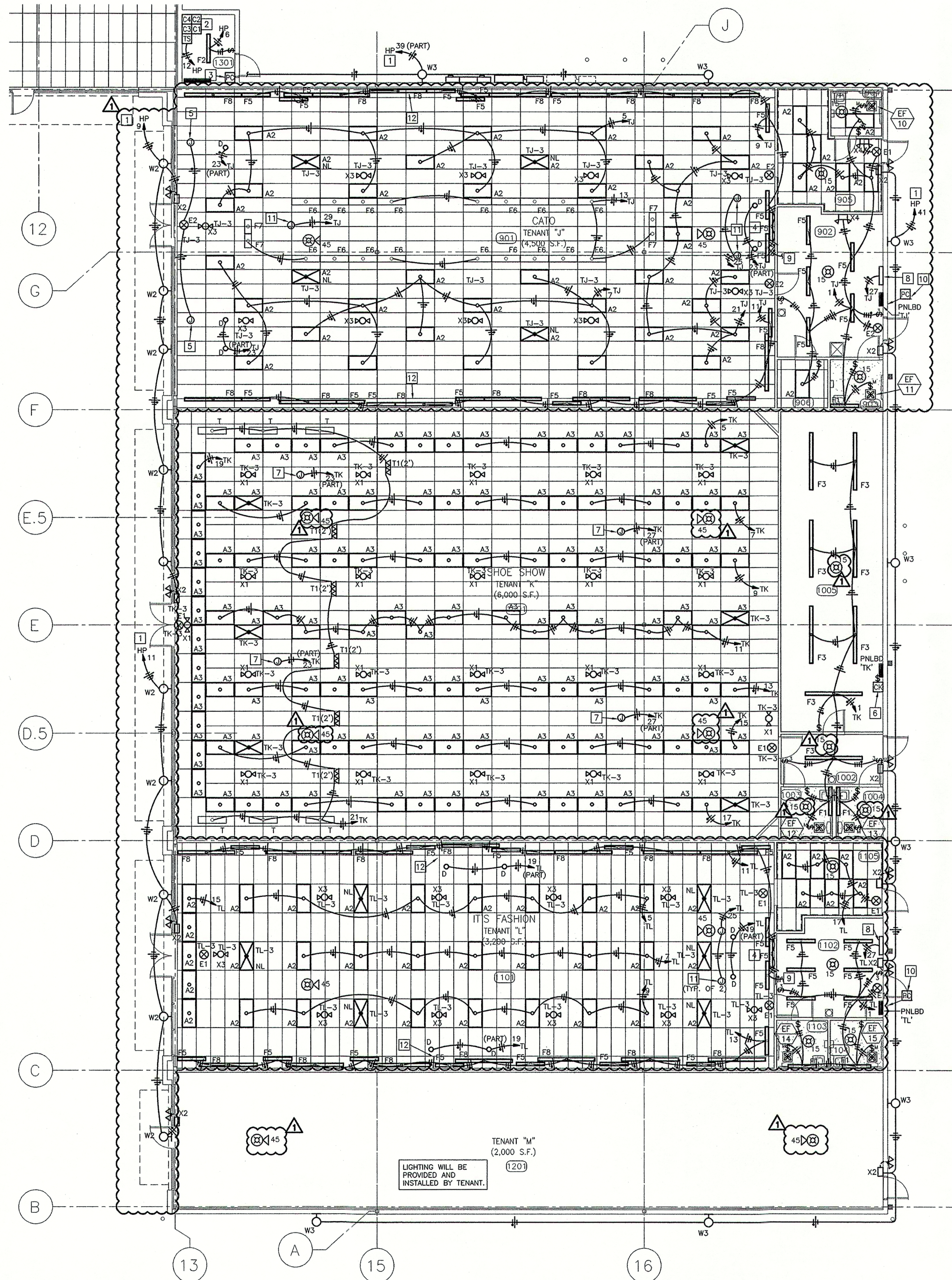
1 LIGHTING FLOOR PLAN SCALE: 1/8"=1'-0"
