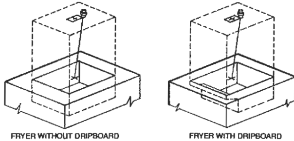
290 NOZZLE TIP POSITIONED OVER THE MIDPOINT OF THE HAZARD AREA ± 3 IN. (7.8 cm) FROM THE MIDPOINT ALONG THE LONGEST SIDE OF THE HAZARD AND ± 1 IN. (2.5 cm) FROM THE MIDPOINT ALONG THE SHORTEST SIDE OF THE HAZARD AND AIMED AT THE MIDPOINT OF THE COOKING AREA.
