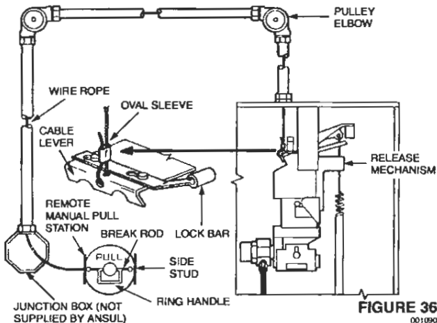
REMOTE MANUAL PULL STATION SINGLE APPLICATION
