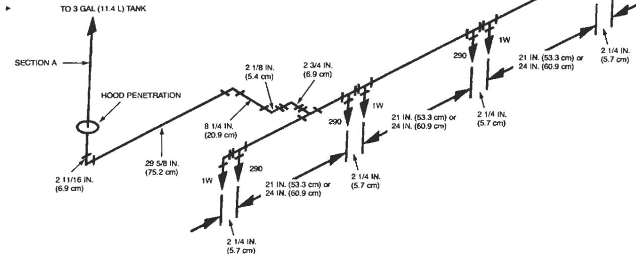
SPECIFIC DISCHARGE PIPING FOR LOW PROXIMITY PROTECTION OF (4) FOUR DEAN INDUSTRIES MODEL GTI GAS FRYERS
