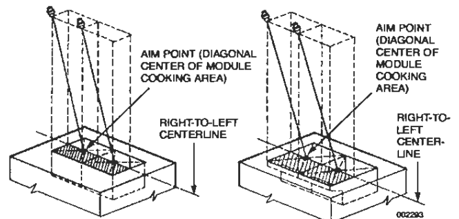
FRYER WITHOUT DRIPBOARD
