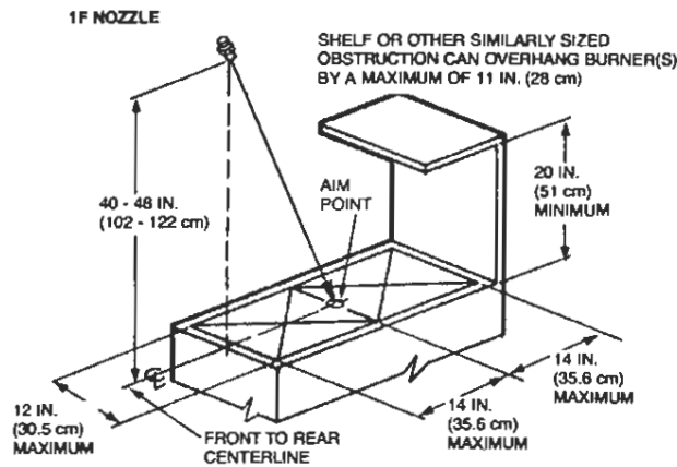
1F NOZZLE LOCATED OVER FRONT EDGE OF BURNER GRATE AND ORIENTED SO NOZZLE TIP FLATS ARE PARALLEL WITH BURNER GRATE FRONT TO REAR CENTERLINE AND SHALL BE AIMED AT THE CENTER OF THE COOKING SURFACE.
