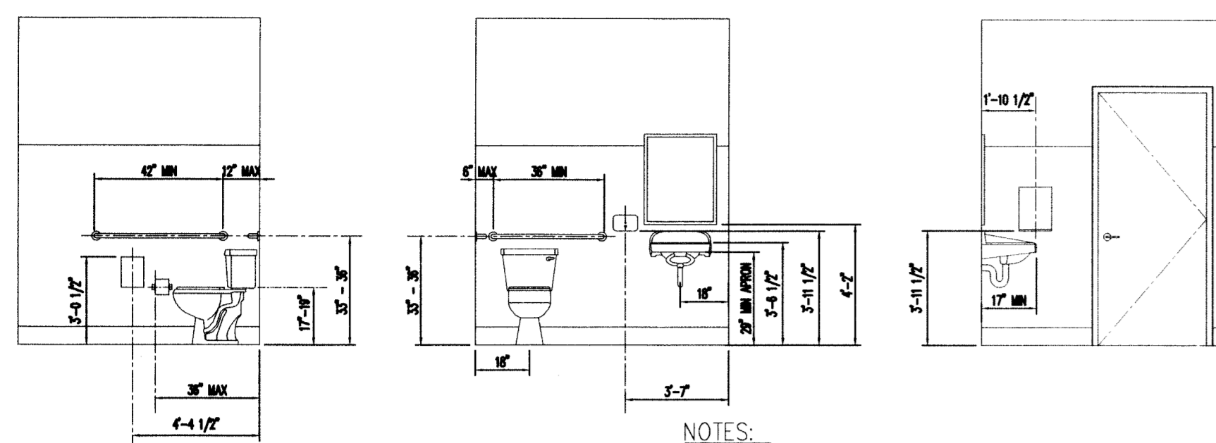
1 RESTROOM ELEVATIONS SCALE: NOT TO SCALE
