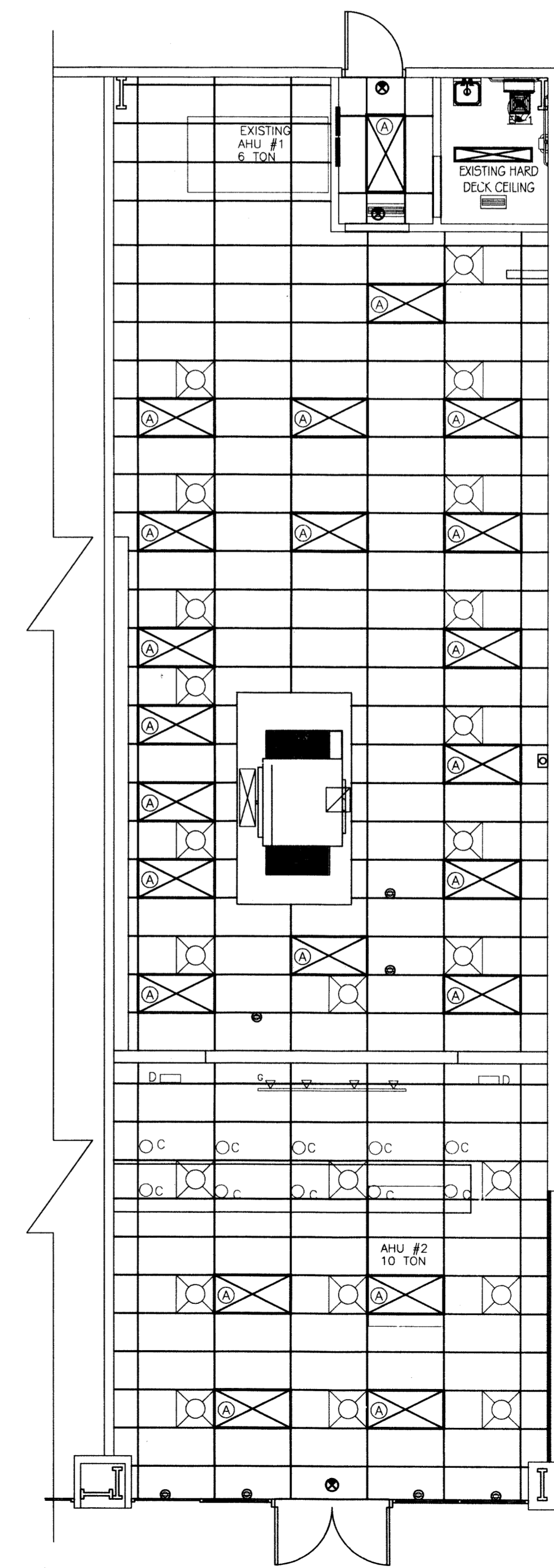
REFLECTED CEILING PLAN SCALE: 3/16" = 1'-0"
