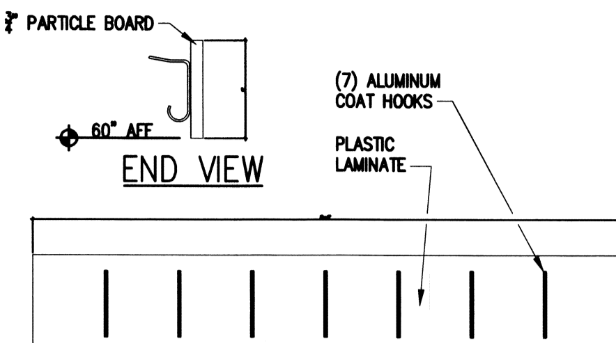
ELEVATION COORDINATE LOCATION WITH OWNER SCALE: N.T.S.
