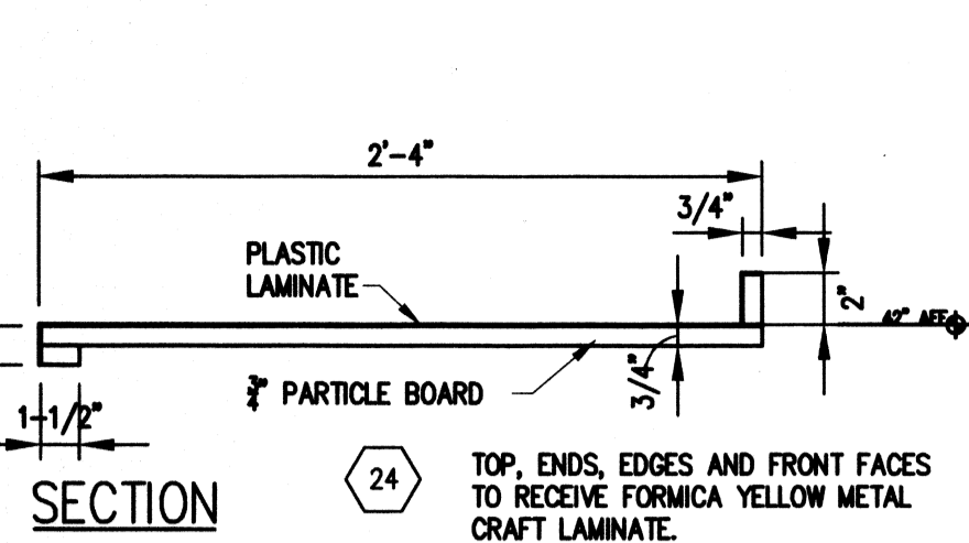
SECTION OFFICE DESK TOP SCALE: 1 1/2" = 1'-0"
