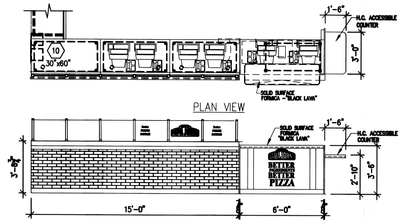
PLAN VIEW FRONT ELEVATION FRONT COUNTER ELEVATION SCALE: N.T.S.
