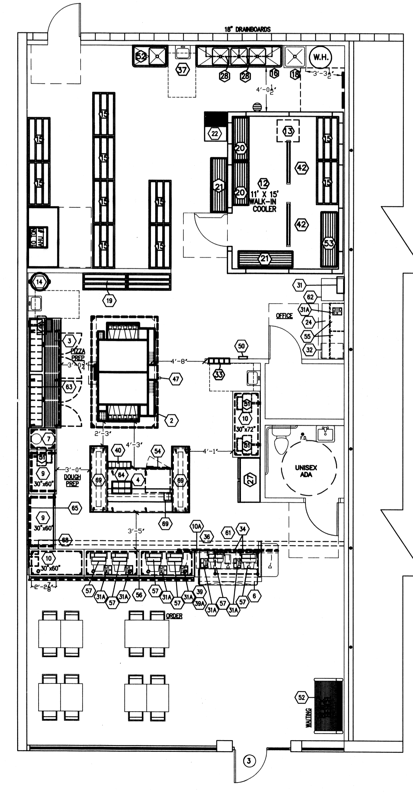
EQUIPMENT PLAN SCALE: 3/16" = 1'-0"
