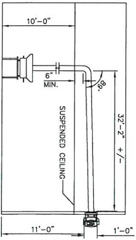
DUCT ROUTING DETAIL ELEVATION N.T.S.
