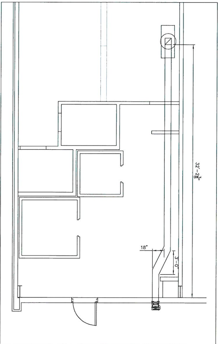
DUCT ROUTING DETAIL PLAN VIEW N.T.S.
