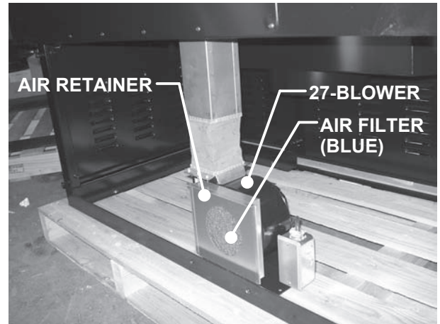
2. The blower is located at the center.
