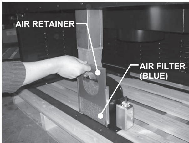
3. Remove the air retainer by pulling it up.
