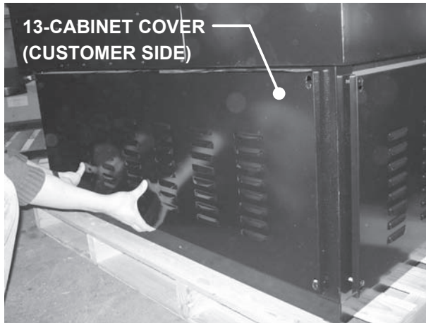
1. Push up from the bottom and pull out the cabinet cover to remove.
