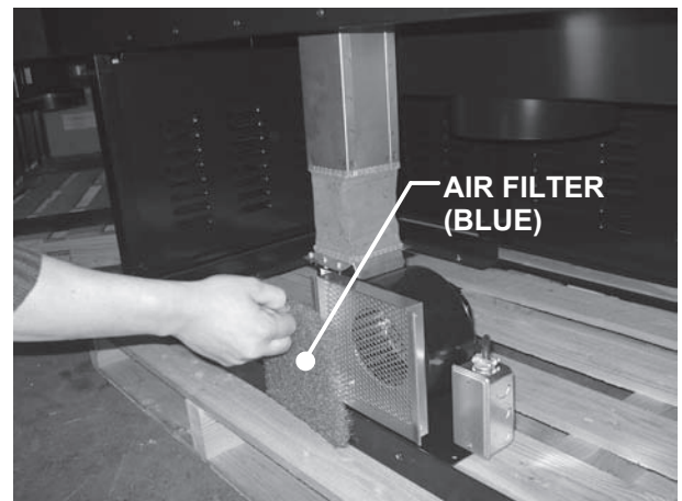
4. Remove the air filter and replace it with a new one.
