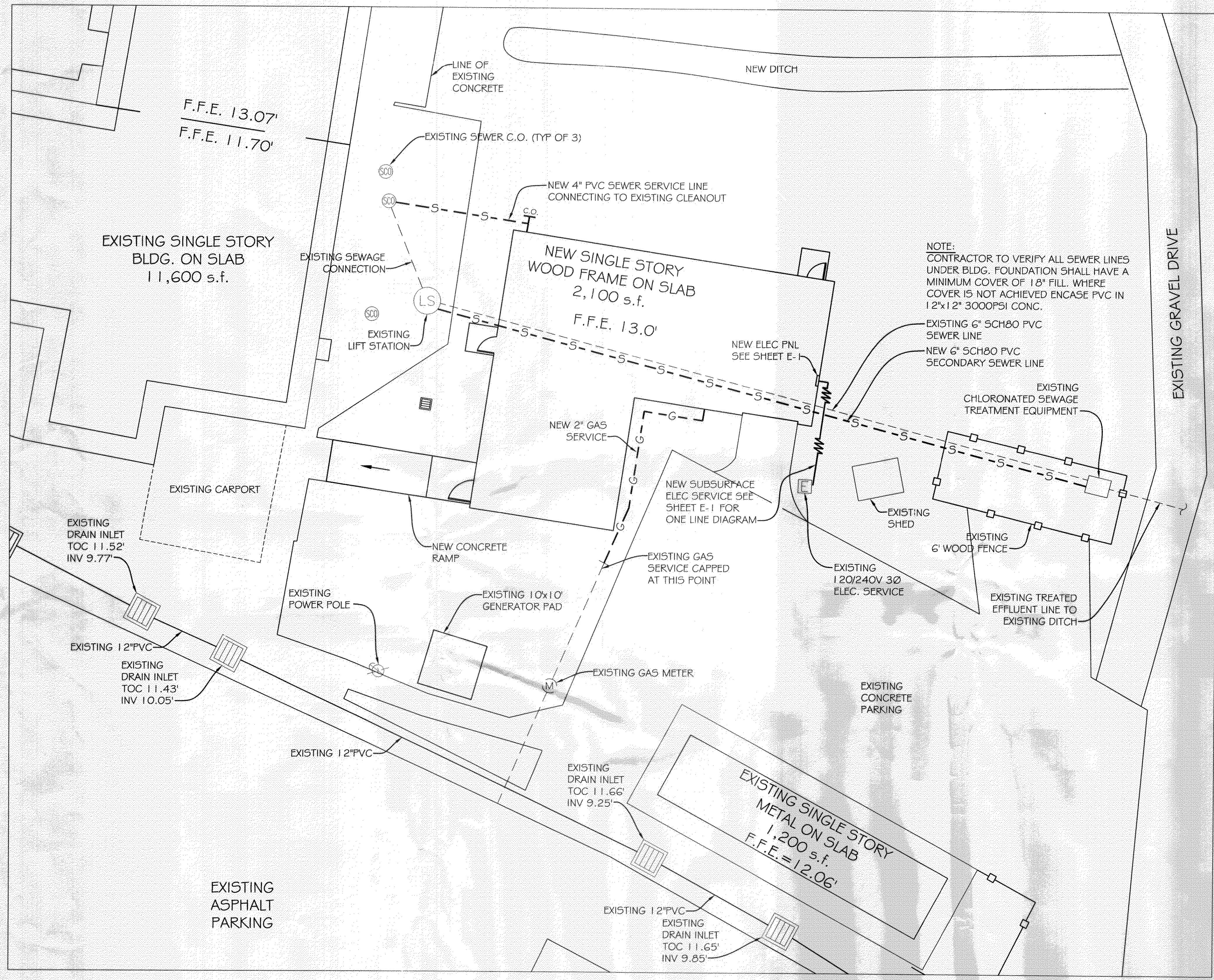
SITE UTILITIES PLAN SCALE: 1" = 10'-0"
