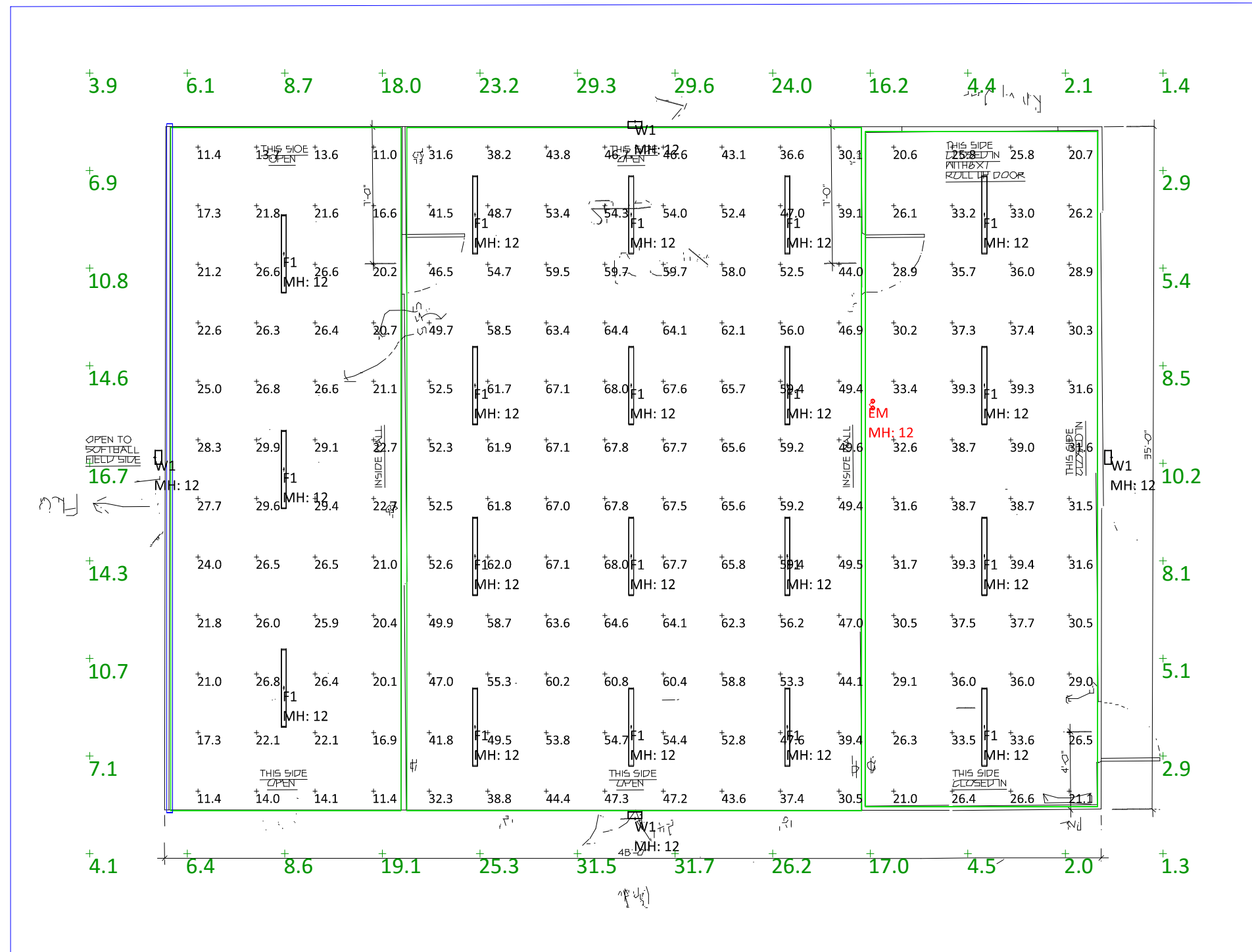
BUILDING FLOOR PLAN SCALE: 1/4" = 1'-0"
