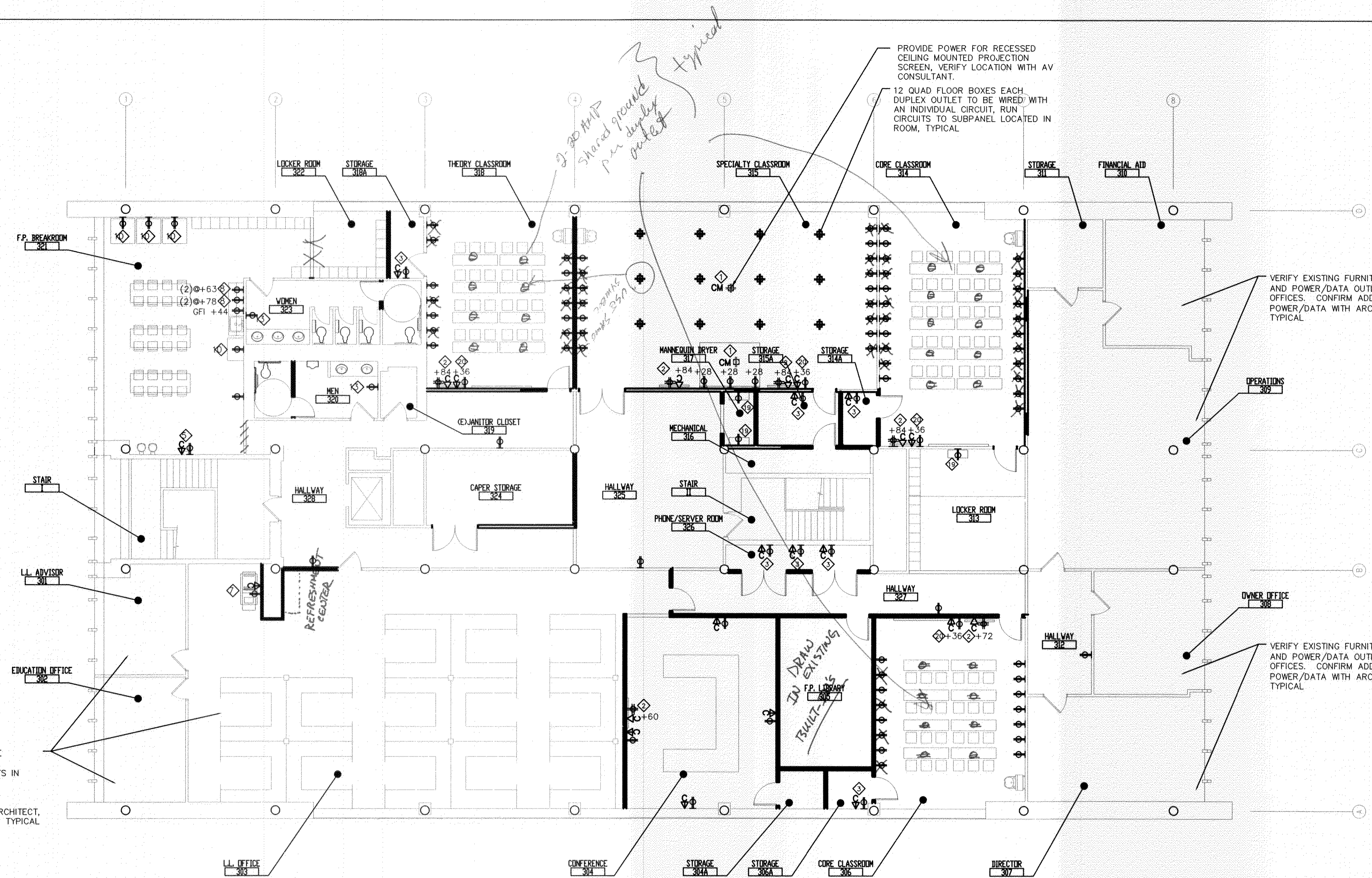
1 POWER LAYOUT PLAN - THIRD FLOOR A 203 SCALE: 1/8"=1'-0"
