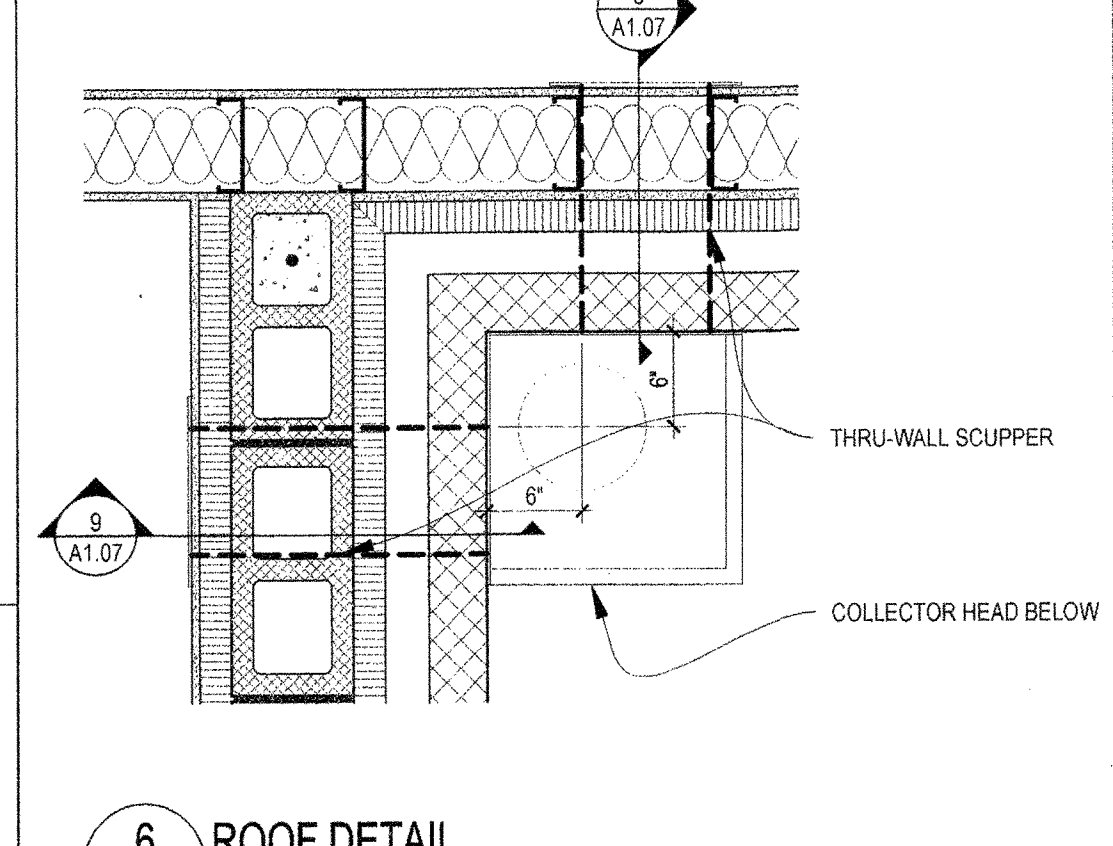
6 ROOF DETAIL A1.06 SCALE: 1" = 1'-0"
