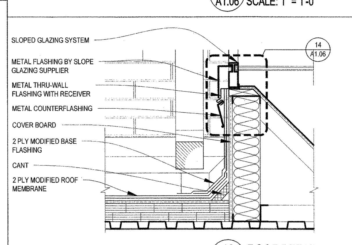
12 ROOF DETAIL A1.06 SCALE: 1" = 1'-0"
