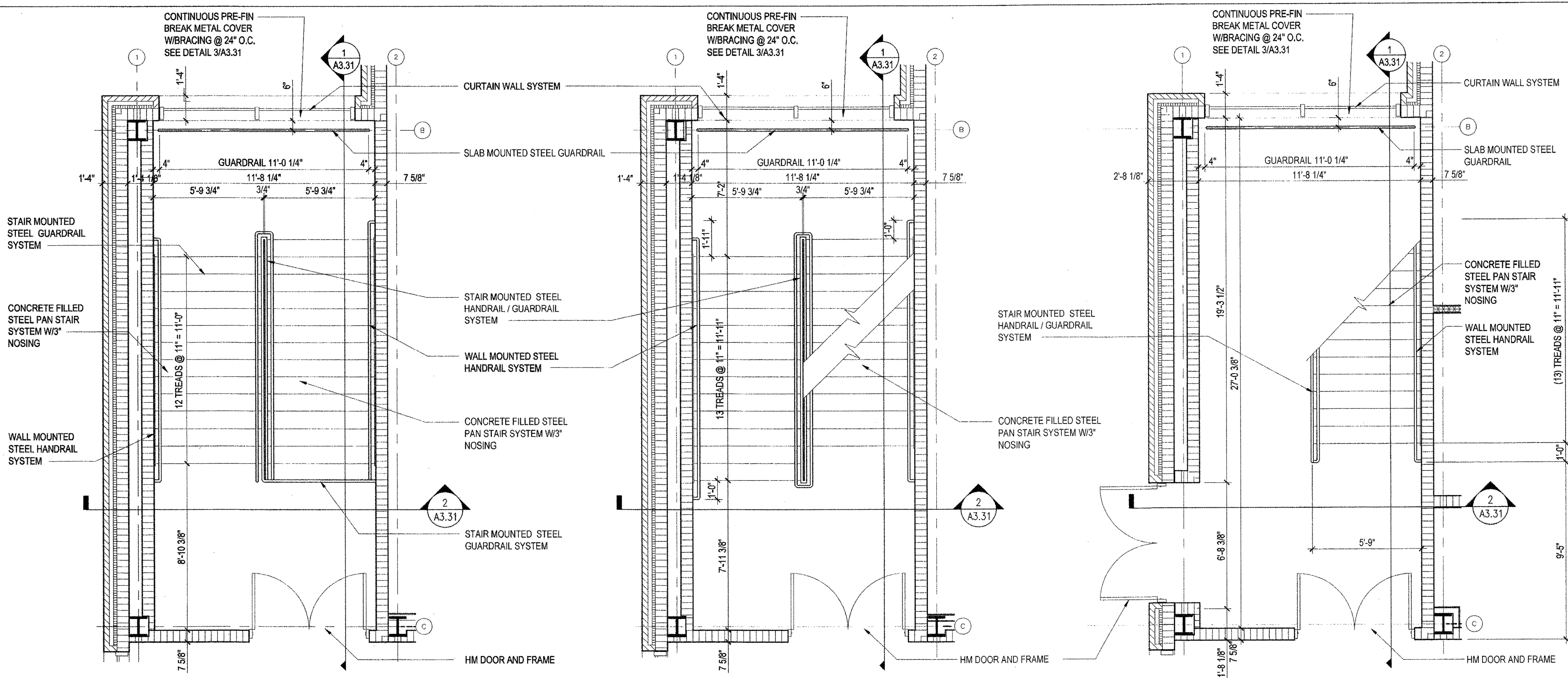
3 UNIT A THIRD FLOOR STAIR S302 A3.21 SCALE: 1/4" = 1'-0"
