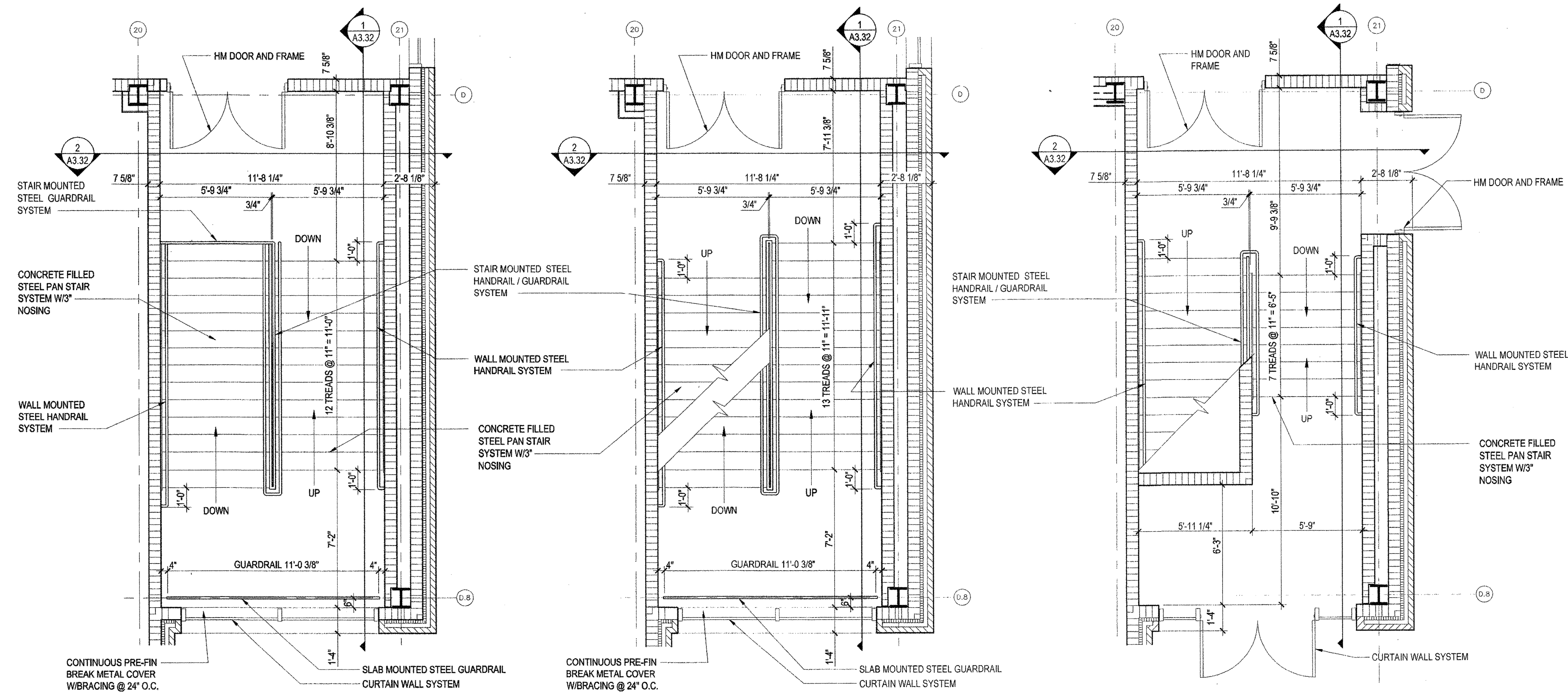
6 UNIT B THIRD FLOOR - STAIR (S301) A3.21 SCALE: 1/4" = 1'-0"
