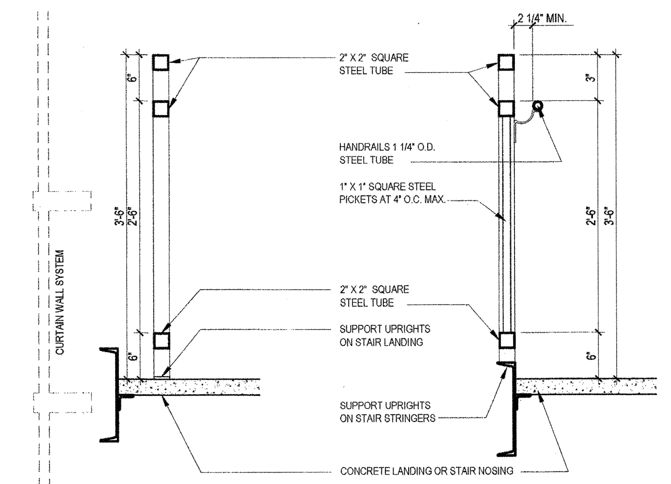
TYPICAL STAIR MOUNTED GUARD RAILS AT CURTAIN WALL TYPICAL STAIR MOUNTED GUARD/HAND RAILS AT RISERS
