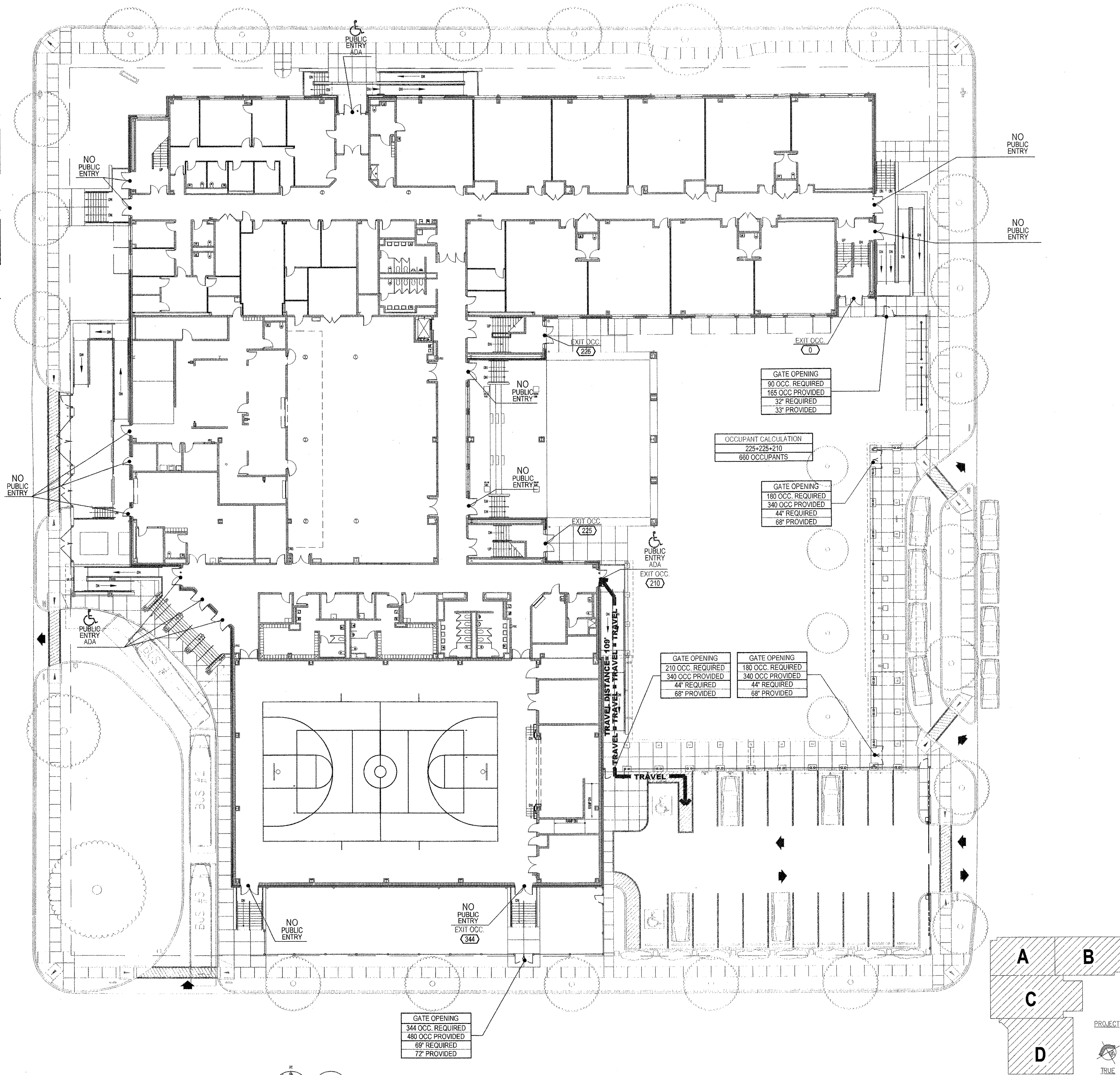
1 SITE - LIFE SAFETY PLAN A0.03 SCALE: NTS
