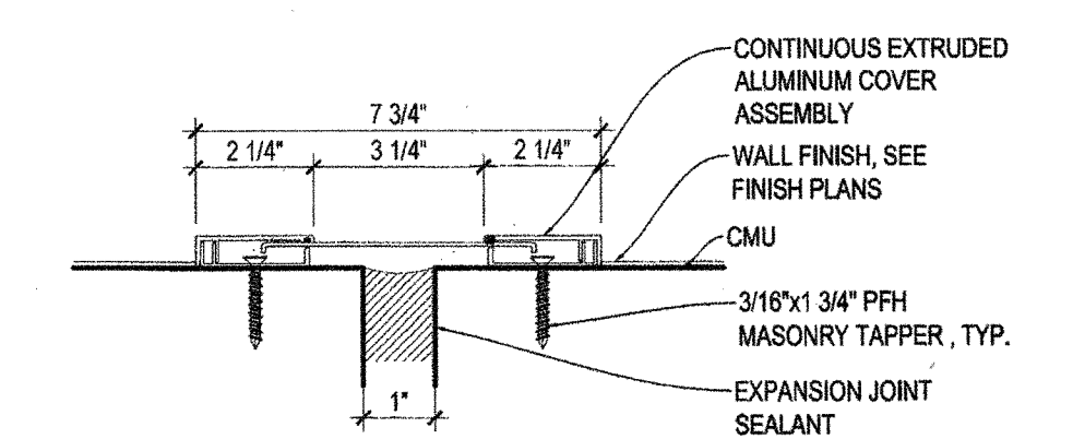
B E.J. WALL-WALL COVER A1.14 / SCALE: 3" = 1'-0"
