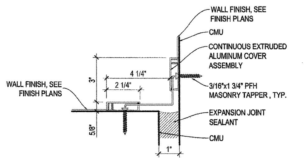
C E.J. WALL-CORNER COVER A1.14 / SCALE: 3" = 1'-0"
