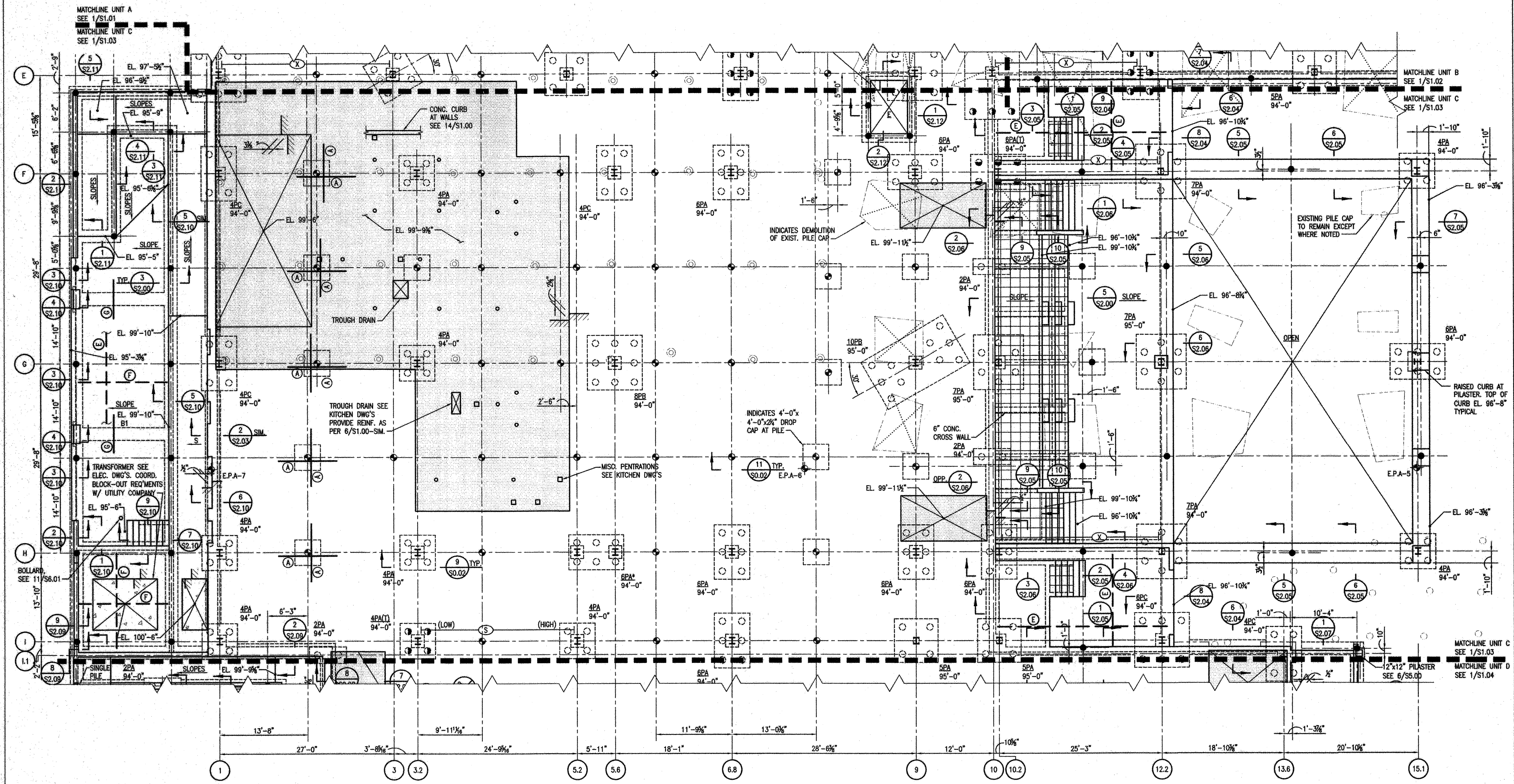
1 PARTIAL FOUNDATION AND FIRST FLOOR FRAMING PLAN S1.03 1/8"=1'-0"
