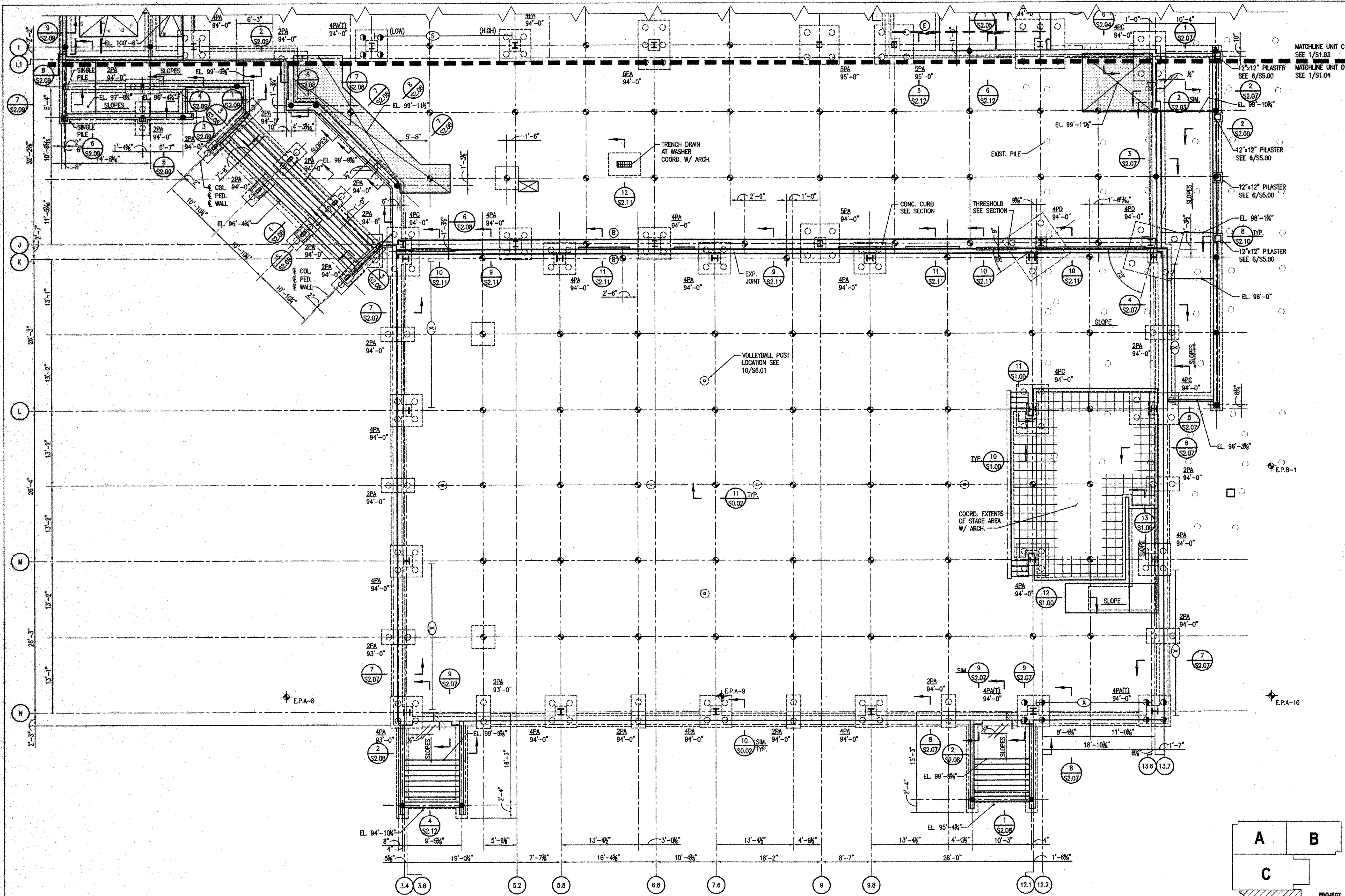
1 PARTIAL FOUNDATION AND FIRST FLOOR FRAMING PLAN S1.04 1/8"=1'-0"
