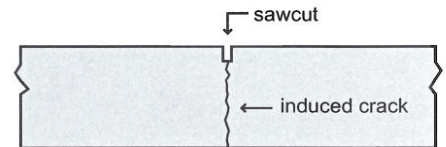
Cross section of contraction joint
