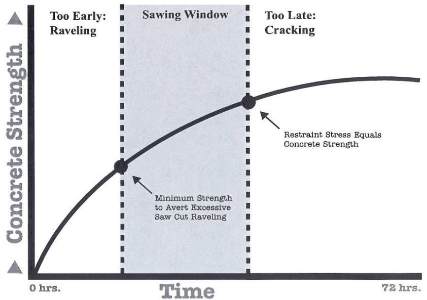
Window of time for sawing
