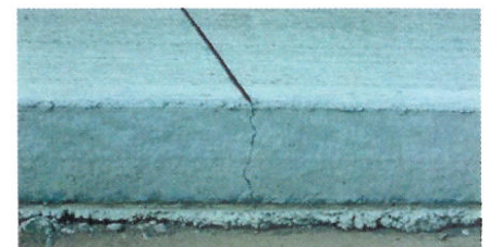
Stop early-age saw cut just short of pavement edge
