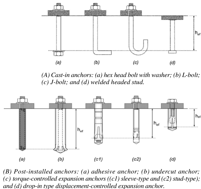
Fig. RD.1.1—Types of anchors.
