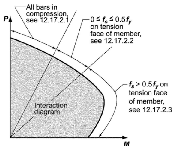
Fig. R12.17—Special splice requirements for columns.
