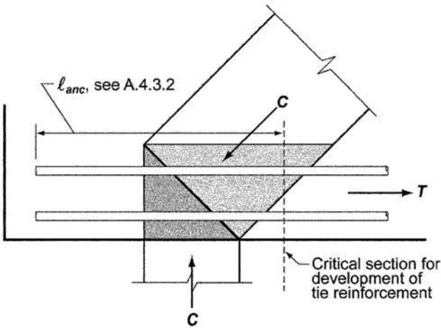
(b) Tension force anchored by a plate
