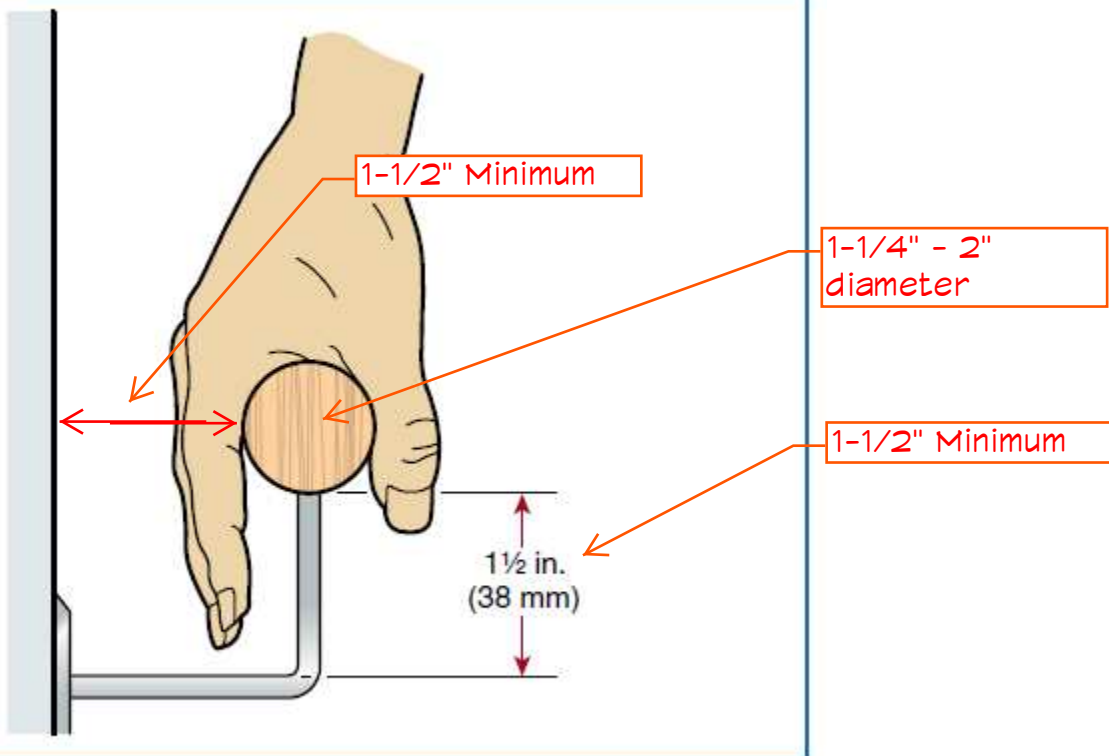
Minimum clearance to handrail brackets.
