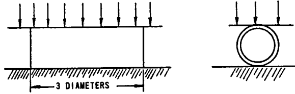
FIG. 14 Crush Test
