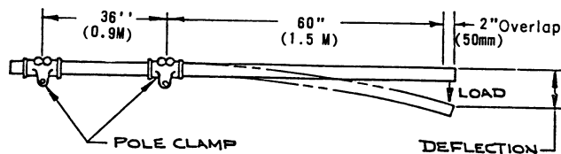
FIG. 13 Bending Deflection Test
