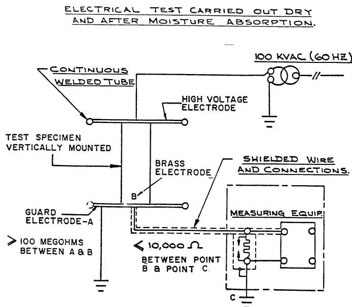
FIG. 3 Typical AC Test Set Up
