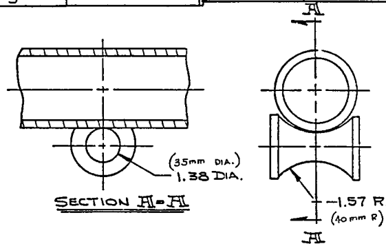
DETAILS OF THE SUPPORTS
