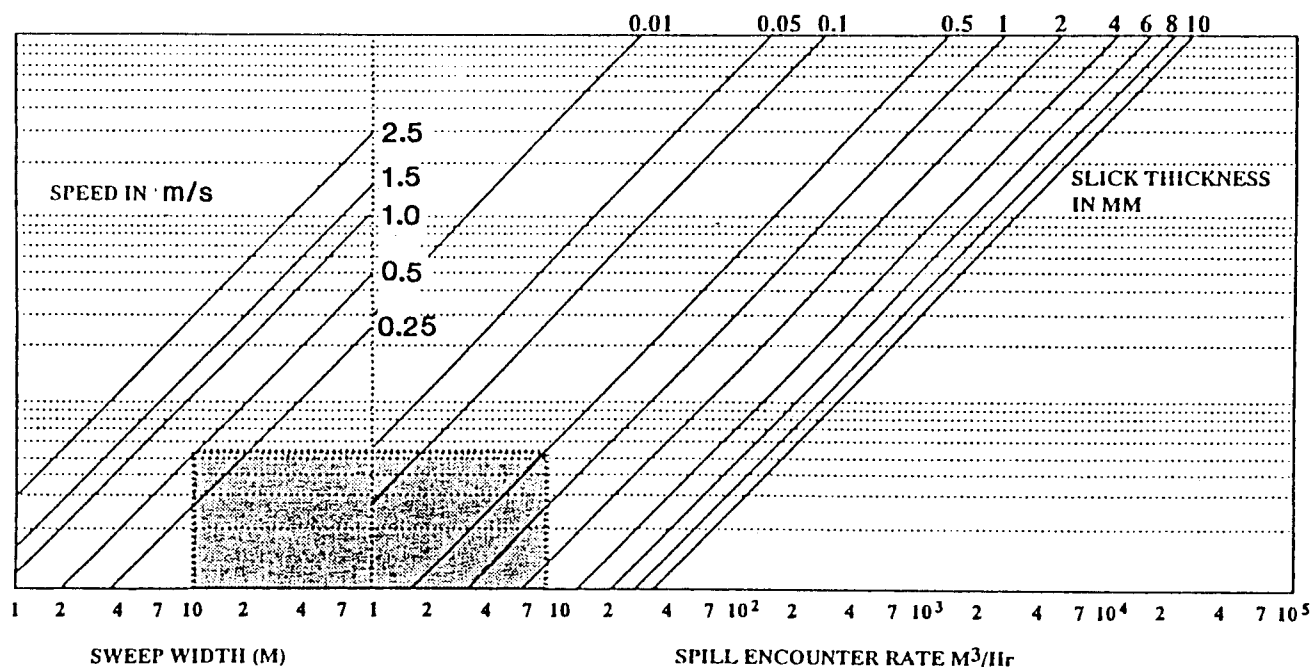
SPILL ENCOUNTER RATE AS A FUNCTION OF SWEEP RATE AND SLICK THICKNESS
