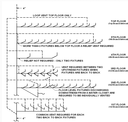
FIGURE 925.C - BATTERY VENTING
