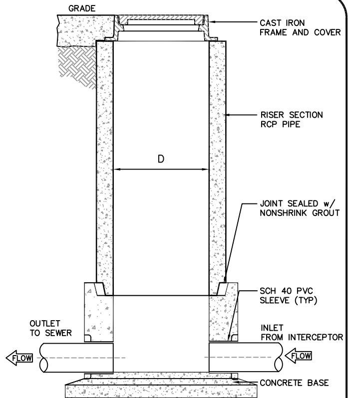
SIDE VIEW
