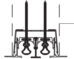
Type 8 CONCEALED PLASTER FRAME CONCEALED MOUNTING
