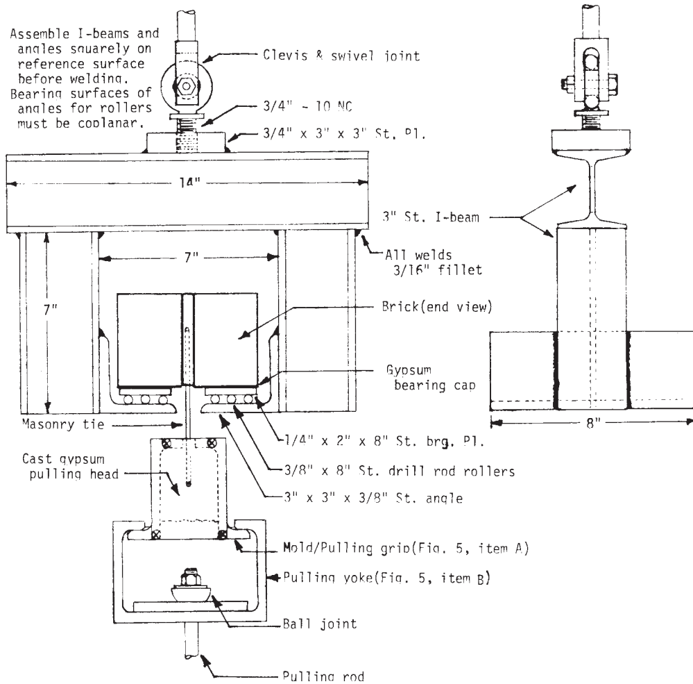
NOTE 1—1 in. = 25.4 mm. FIG. 2 Procedure A Apparatus and Setup
