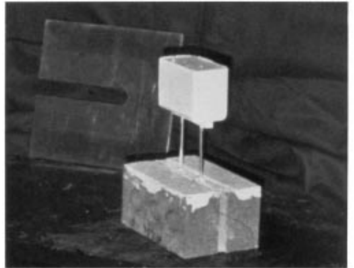
FIG. 5 Notched Metal Plate Used for Capping Specimens in Procedure A
