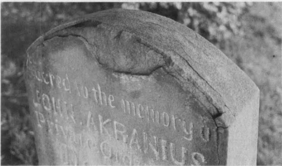
Delamination of sandstone along the bedding planes. Photograph: U.S. Corps of Engineers.
