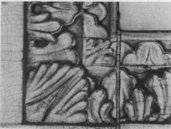
Crazing of glazed terra cotta. Photograph: National Park Service.
