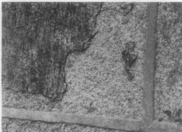
Peeling of granite. Photograph: Baird M. Smith, AIA.
