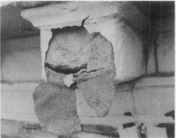
A neoprene coating over a limestone cornice has trapped water (which entered through leaks in the parapet) inside these stone dentils. The built-up water pressure has finally forced the coating to pop off, taking with it pieces of the stone. Photograph: National Park Service.
