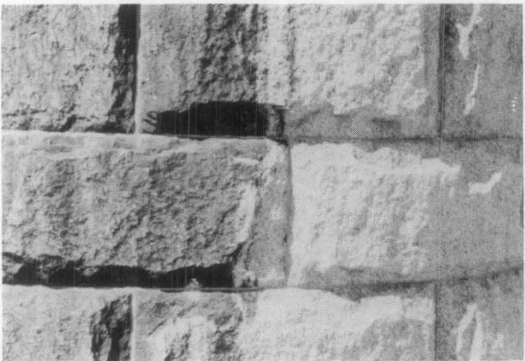
Chemical cleaning to remove urban dirt and pollution from granite without causing damage or abrasion to the surface of the stone.
