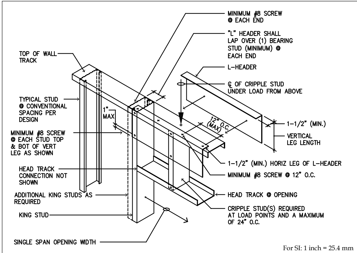
Figure C2-1 Double L-Header
