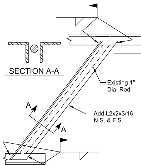
Fig. 17. Angles and welds added.
