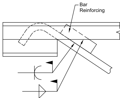
Fig. 18. Bar added for additional weld.
