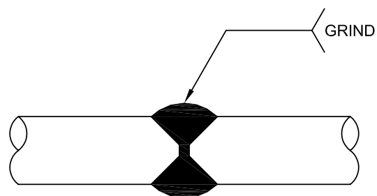
Fig. 2f. Rod splice.
