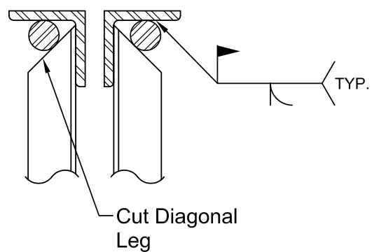
Fig. 2e. Top chord reinforcement—rods.
