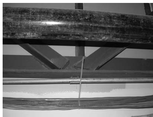
Fig. 14. Web angles on side of chords.
