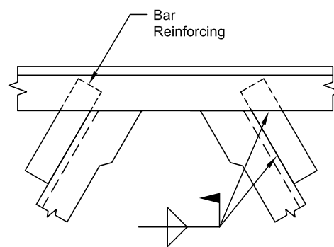
Fig. 10. Reinforcing diagonals.
