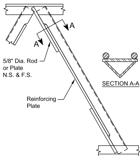
Fig. 9. Crimped web reinforcement.
