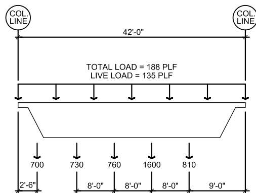
Fig. 19. Joist loading.
