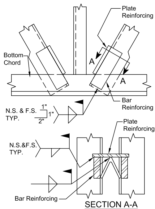
Fig. 11. Reinforcing diagonals.
