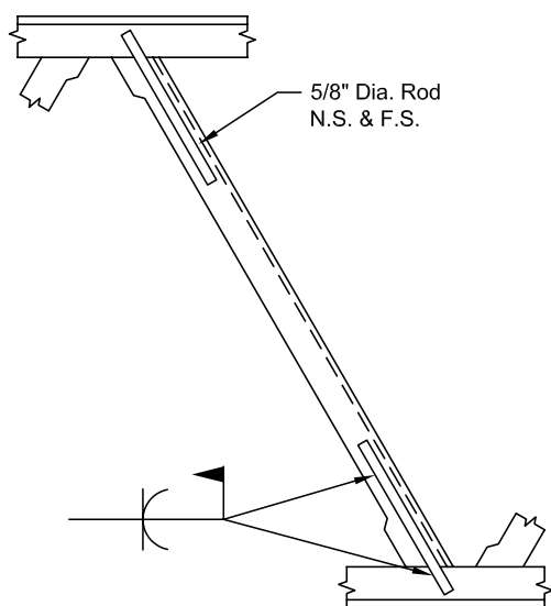
Fig. 8. Weld-only reinforcement.
