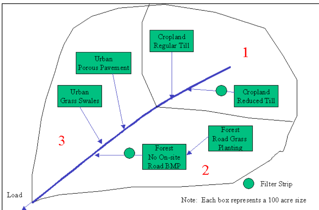
Figure A10. Case that needs the BMP Calculator. You need to calculate the combined BMP efficiency because each land use type uses more than one practice (e.g., regular till and reduced till combined with filter strips for cropland). In this example, you need to calculate a combined efficiency for each land use type or subwatershed.
