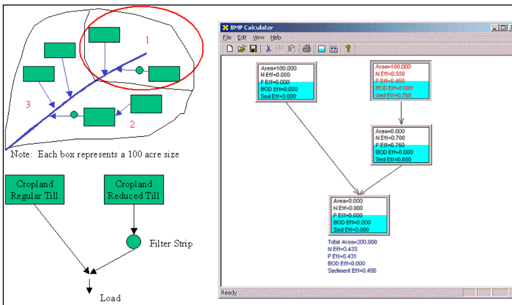
Figure A11. Calculation of combined BMP efficiency for sample cropland. For Area 1 in the watershed, one-half of the cropland uses no BMPs and the other half uses reduced tillage practice and a filter strip in a serial configuration. The two halves of the cropland are arranged in a parallel configuration. Because the filter strip is represented in the BMP Calculator as a box that is separated from the filter strip's treatment area, the source area for the filter strip itself equals zero.
