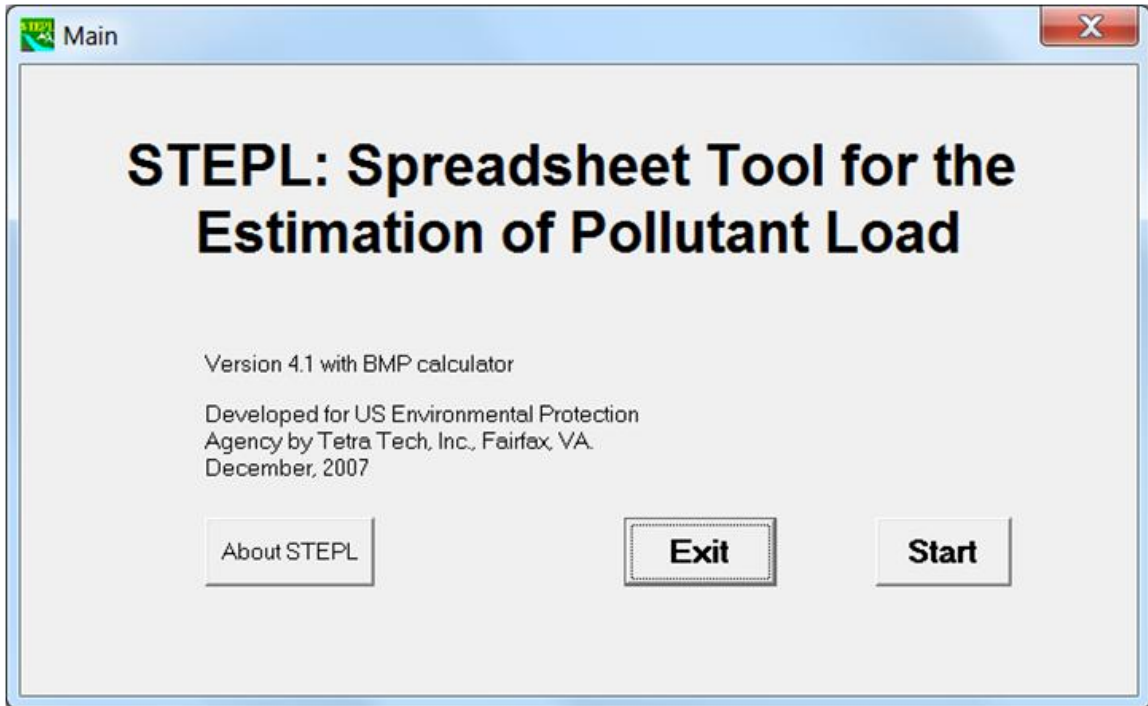
Figure 3. Main program.
