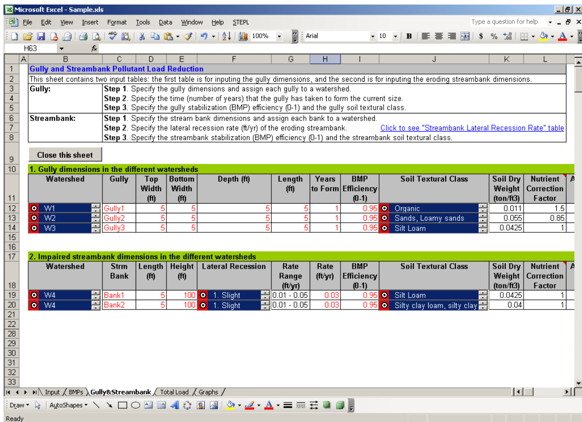
Figure 13. The Gully&Streambank worksheet, which lets you define the dimensions, BMP efficiency, and soil textural class for the gully formation and impaired streambank with in the selected watershed. Note that for this example, there are user-defined three gully formations and two impaired streambanks.
