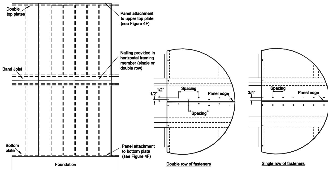
Figure 4H Panel Splice Occurring across Studs
