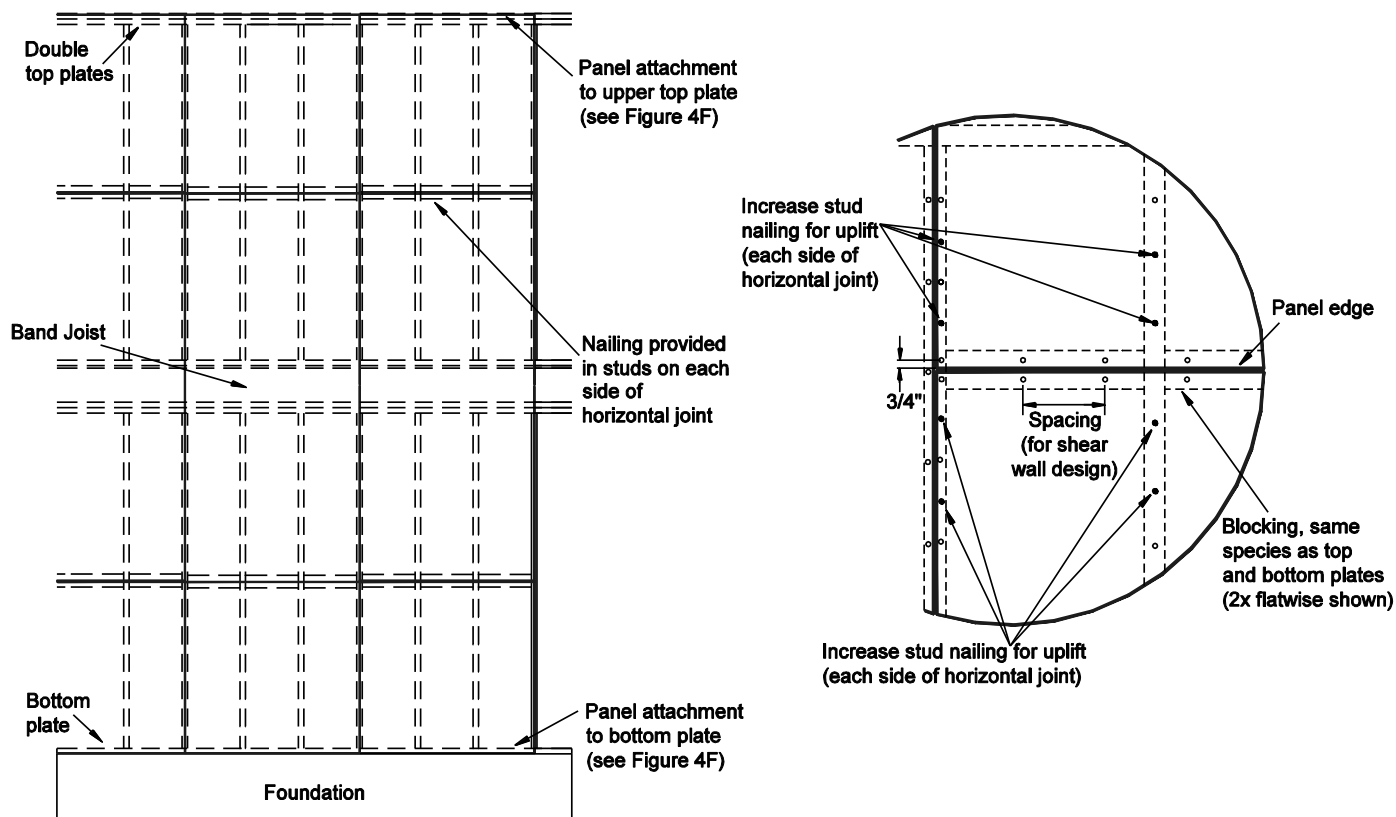
Figure 4H Panel Splice Occurring across Studs
