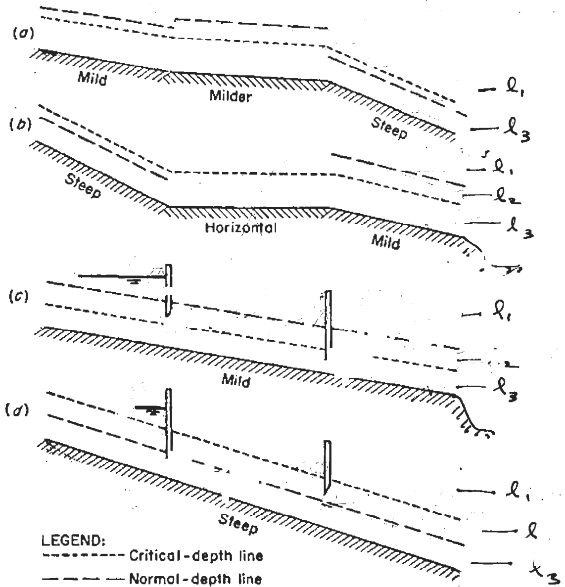
FIG. 9-13. Channels for Prob. 9-7. The vertical scale is exaggerated.
