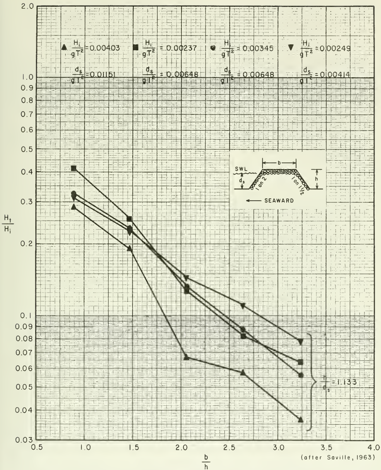
Figure 7-55. Monochromatic wave transmission, permeable rubble-mound breakwater, where \frac{h}{d_s} = 1.33 .
