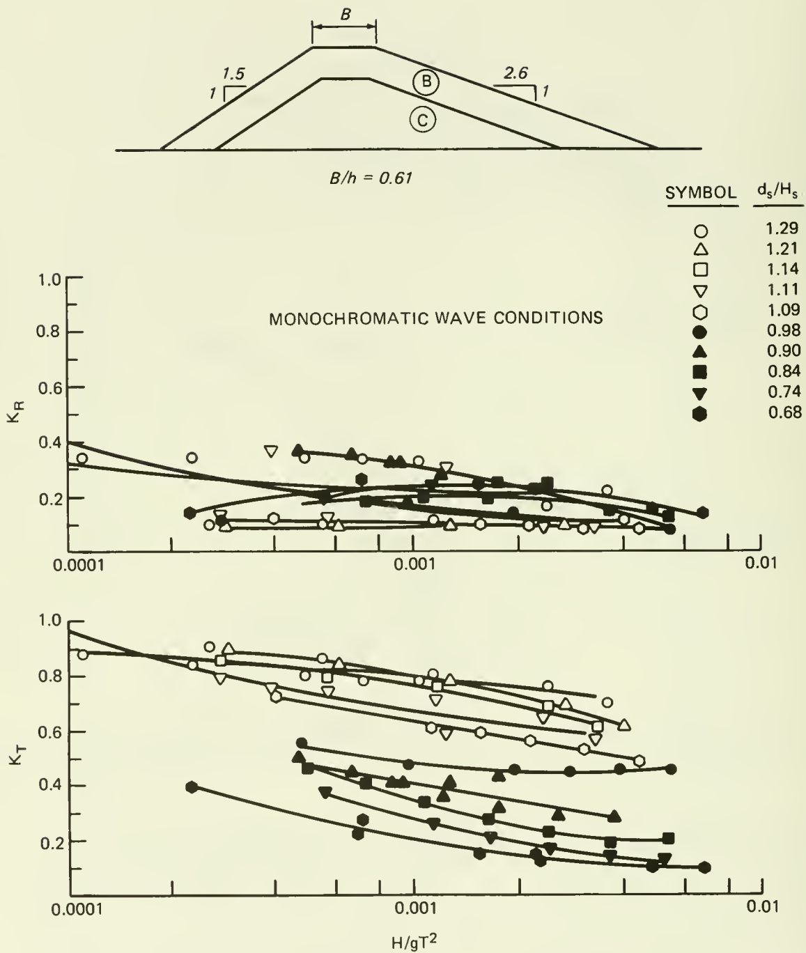
Figure 7-52. Wave transmission and reflection coefficients for a breakwater with a flat seaward slope in medium-depth water ( d/gT^2 \approx 0.015 ).
