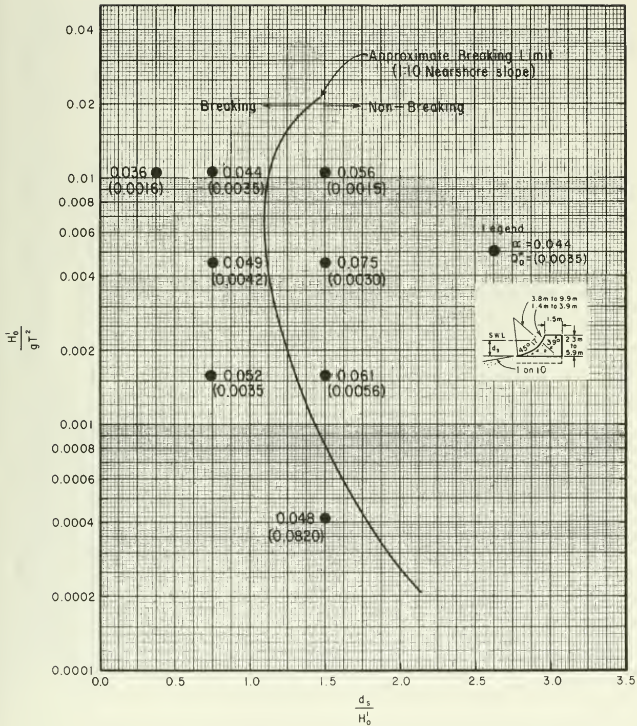
Figure 7-30. Overtopping parameters \alpha and Q_o^* (curved wall on a 1:10 nearshore slope).
