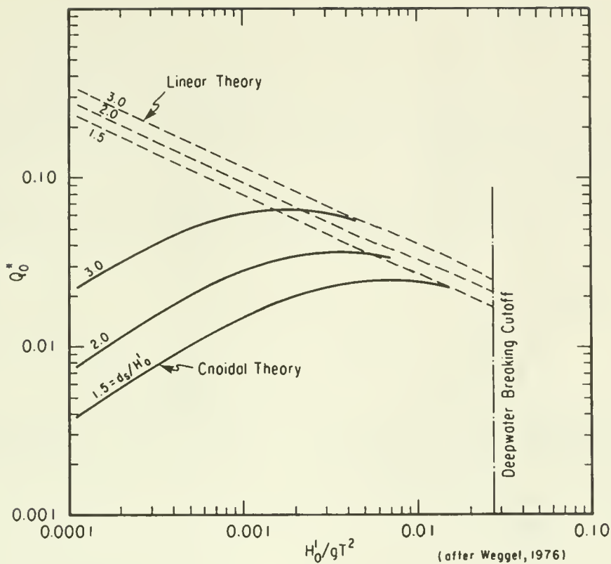
Figure 7-34. Variation of Q_o^* between waves conforming to cnoidal theory and waves conforming to linear theory.
