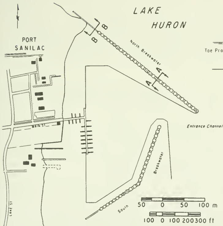
Figure 6-65. Cellular-steel sheet-pile and sheet-pile breakwater.
