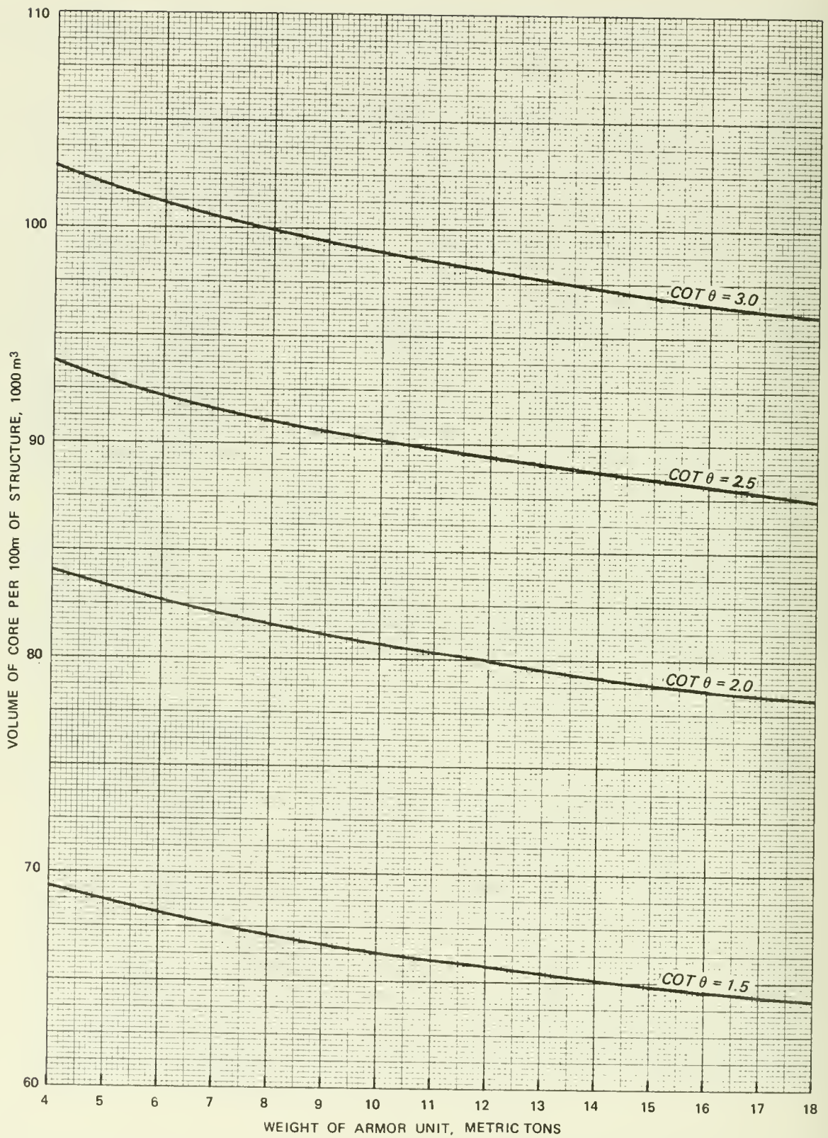
Figure 8-27. Volume of core per 100 meters of structure as a function of armor unit weight and structure slope.
