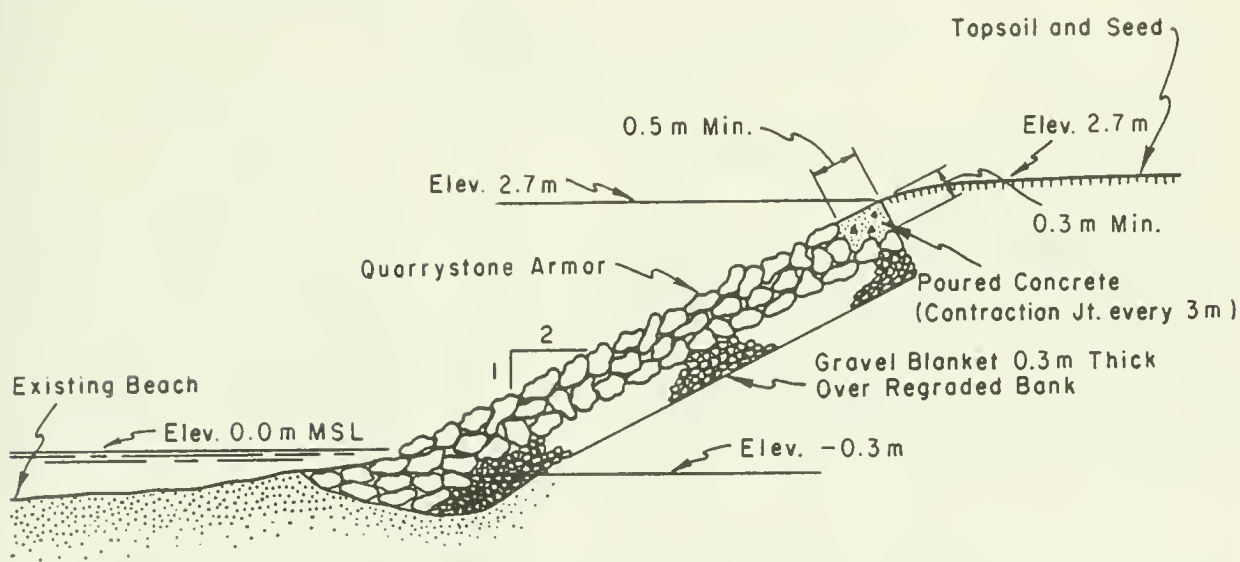
Figure 6-10. Quarrystone revetment.
