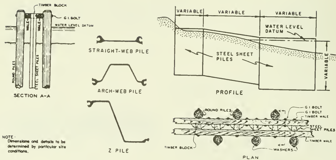
Figure 6-55. Timber-steel sheet-pile groin.
