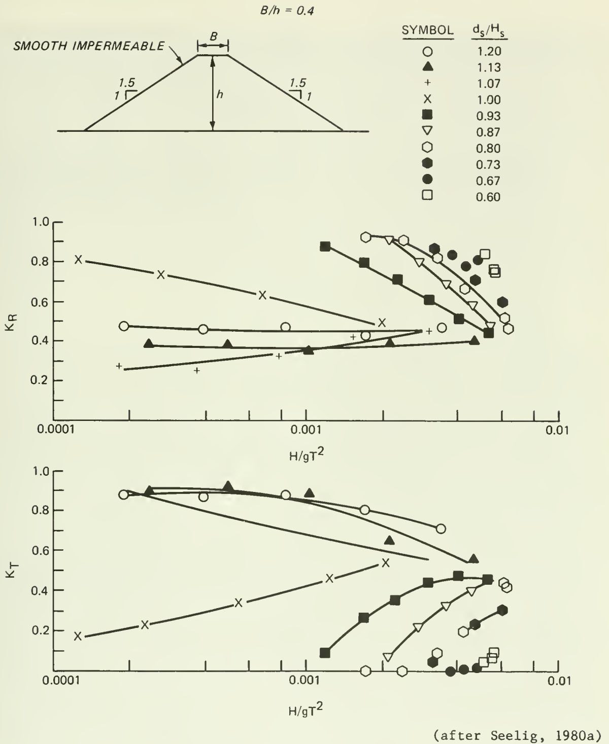
Figure 7-46. Sample wave transmission and reflection coefficients for a smooth, impermeable breakwater.
