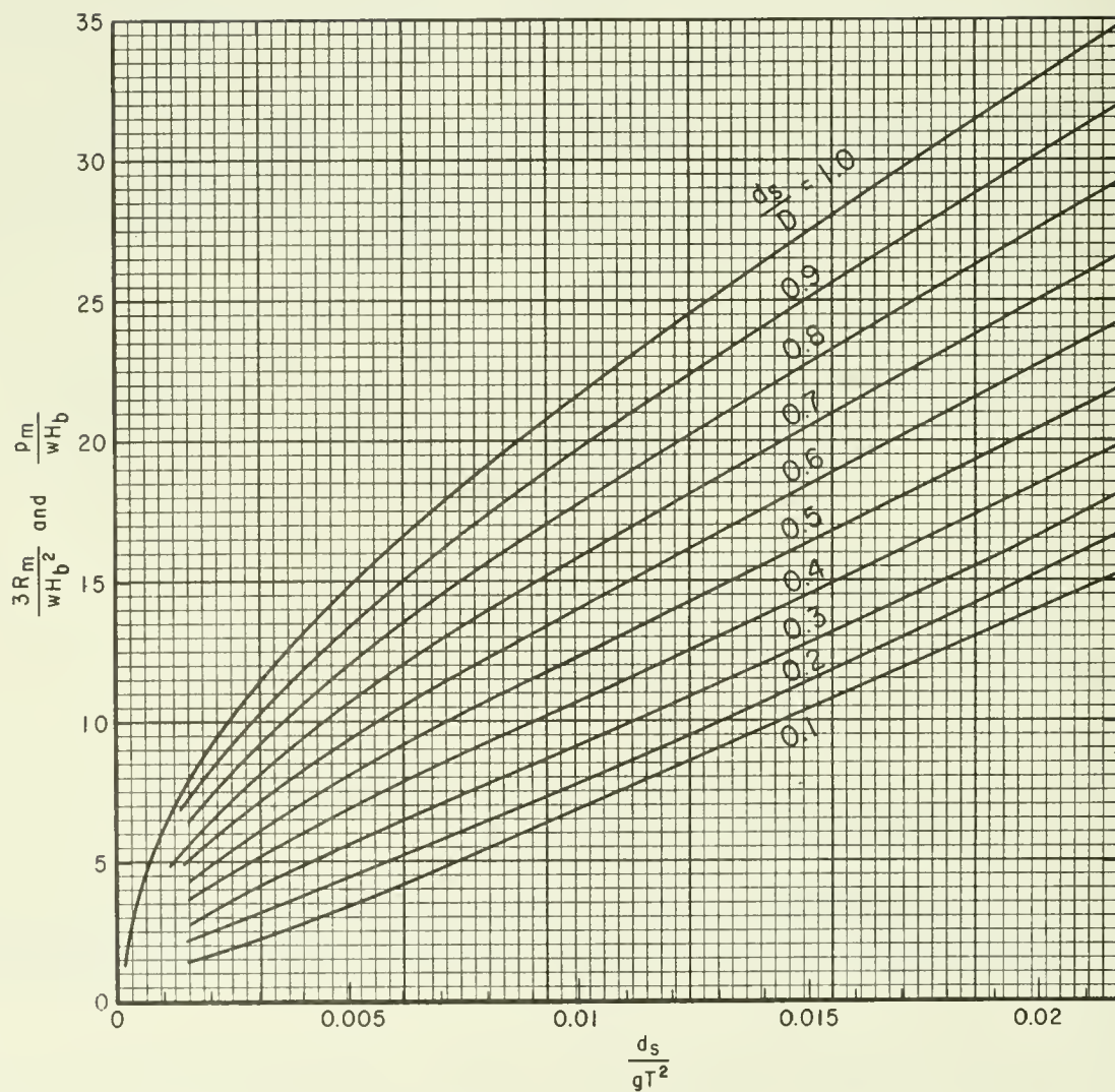
Figure 7-101. Dimensionless Minikin wave pressure and force.
