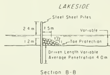
TYPICAL SECTIONS OF BREAKWATER
