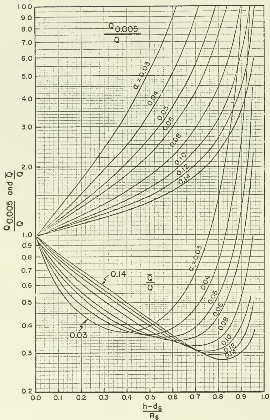
Figure 7-35. \frac{Q_{0.005}}{Q} and \frac{h-d_s}{R_s} as functions of relative freeboard and \alpha .
