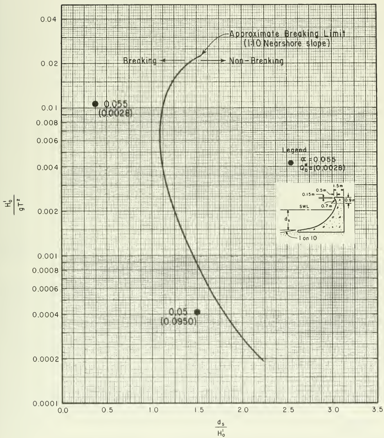
Figure 7-32. Overtopping parameters \alpha and Q_O^* (recurved wall on a 1:10 nearshore slope).
