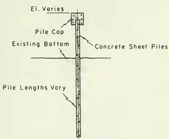
Figure 6-58. Prestressed-concrete sheet-pile groin.
