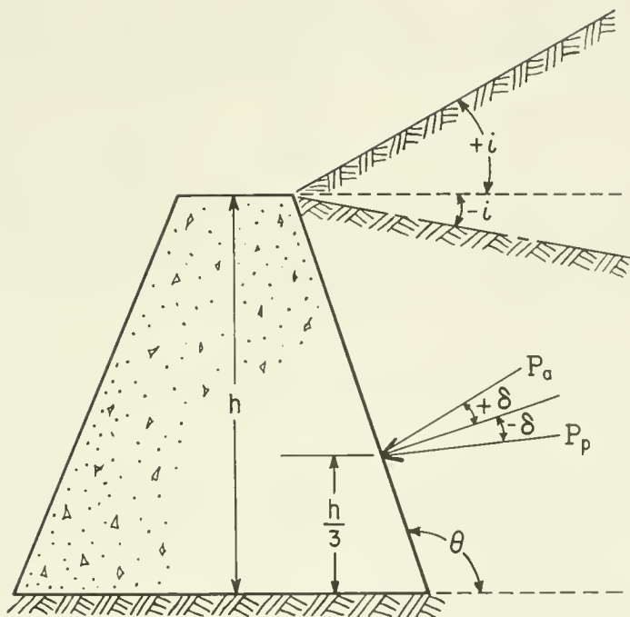
Figure 7-122. Definition sketch for Coulomb earth force equation.
