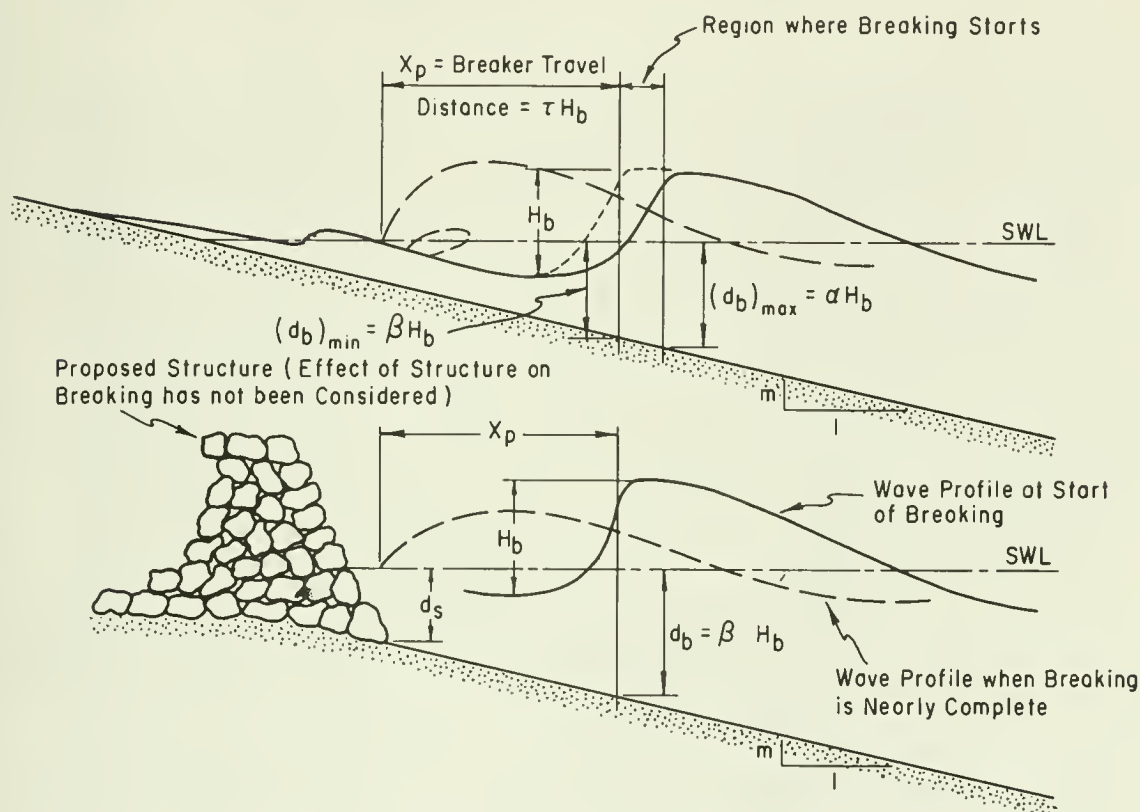
Figure 7-1. Definition of breaker geometry.
