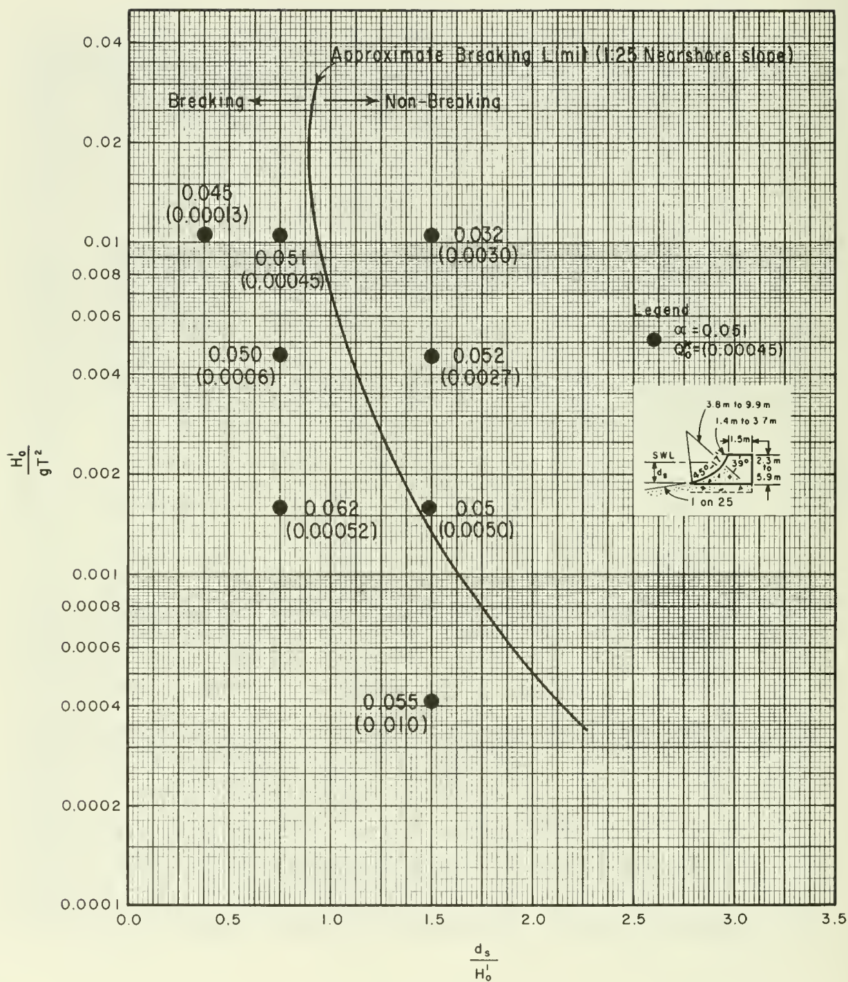
Figure 7-31. Overtopping parameters \alpha and Q_o^* (curved wall on a 1:25 nearshore slope).
