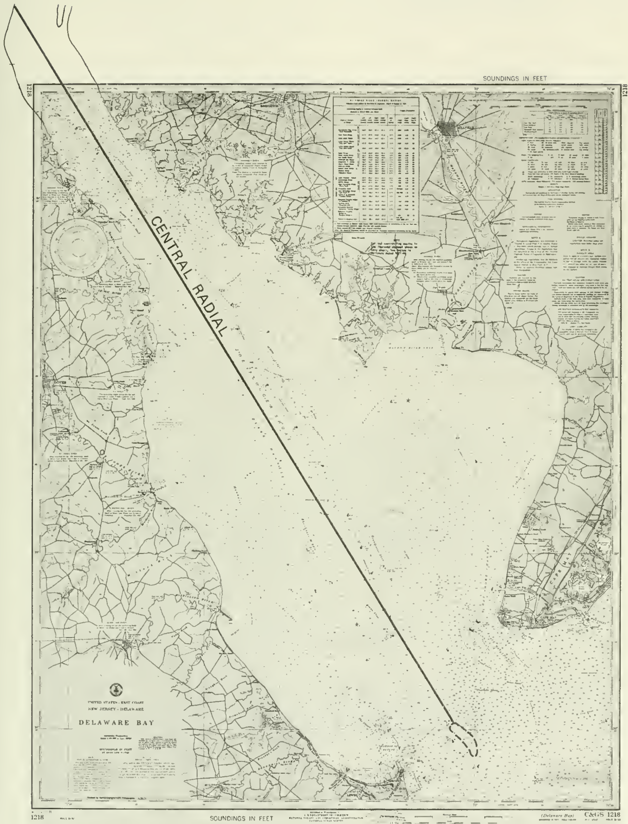
Figure 8-11. Determination of longest fetch: island site at Delaware Bay entrance.
