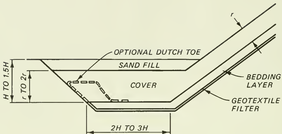
BURIED TOE APRON
