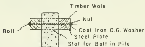
TIMBER WALE
