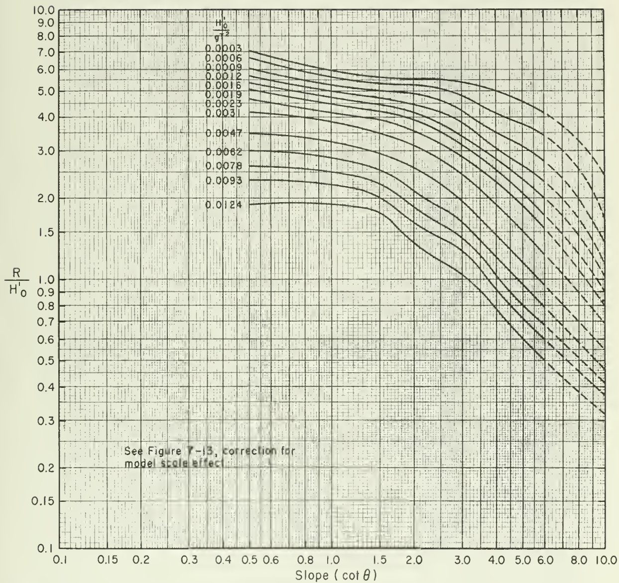
Figure 7-10. Wave runup on smooth, impermeable slopes when \frac{d}{s H_0} \approx 0.80 (structures fronted by a 1:10 slope).
