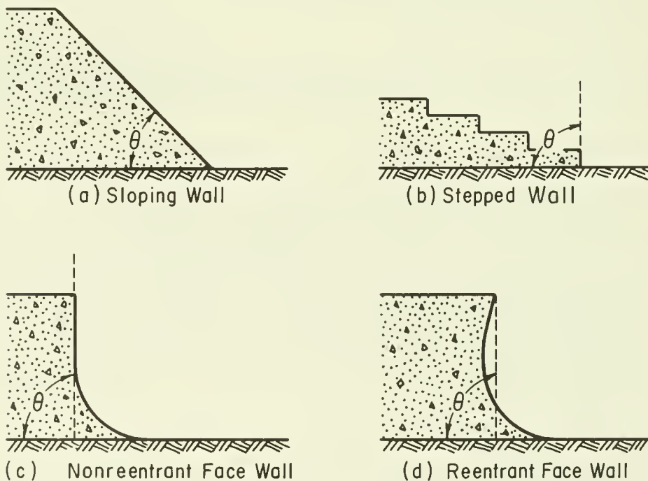
Figure 7-107. Wall shapes.
