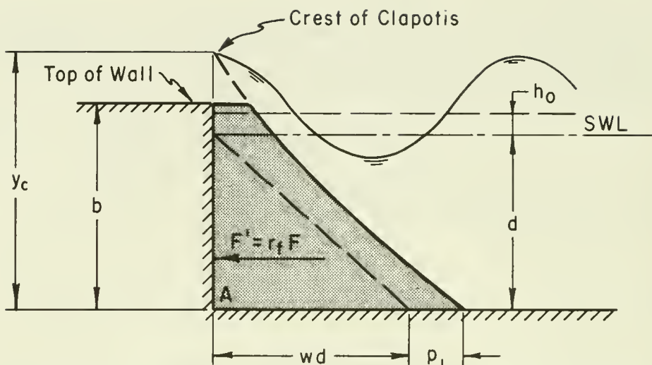
Figure 7-96. Pressure distribution on wall of low height.
