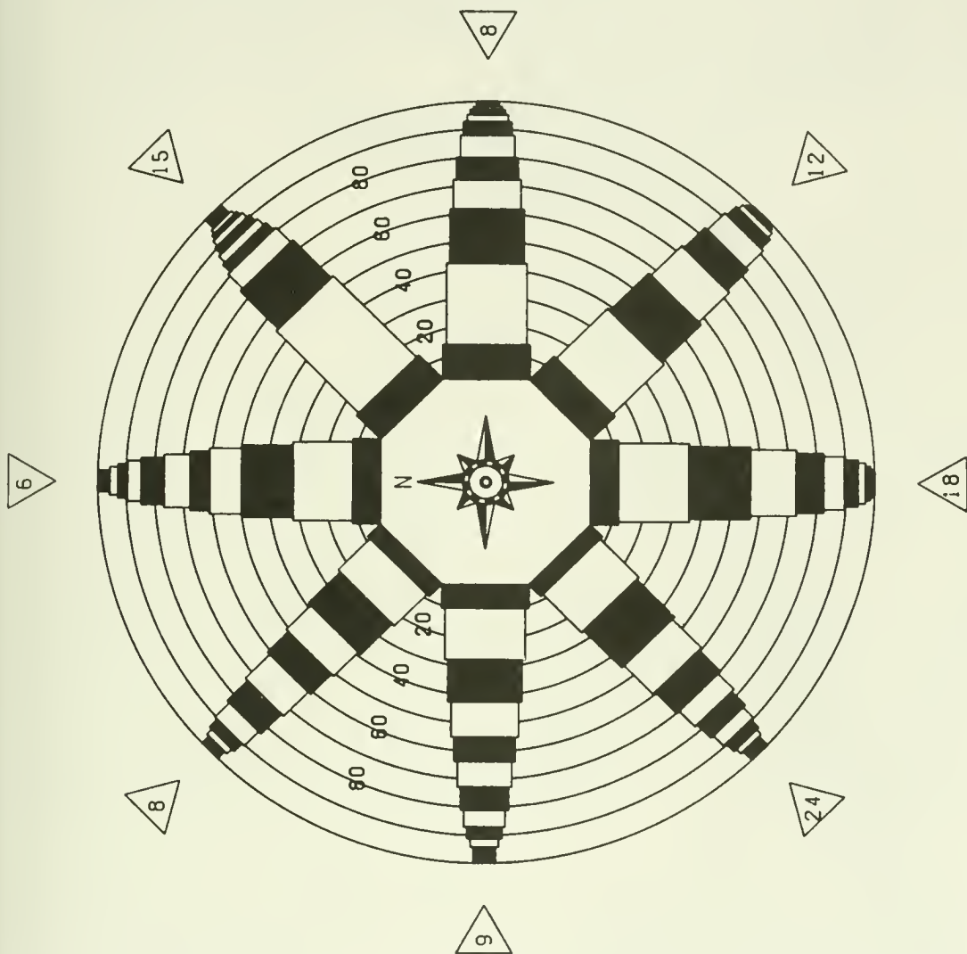
Figure 8-16. Wave diagram for station 4 off the Delaware Bay entrance (numbers within concentric rings are percent of waves of different height occurring from each direction; numbers in triangles represent percent of time waves occur in each direction).
