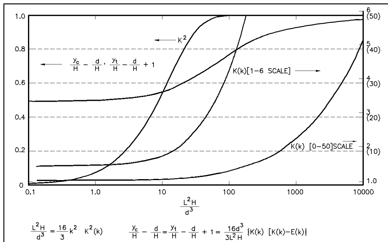
Figure II-1-14. Relationship among L^2 H/d^3 and the square of the elliptic modulus ( k^2 ), y_c/H , y_t/H , and K(k) (Wiegel 1960)
