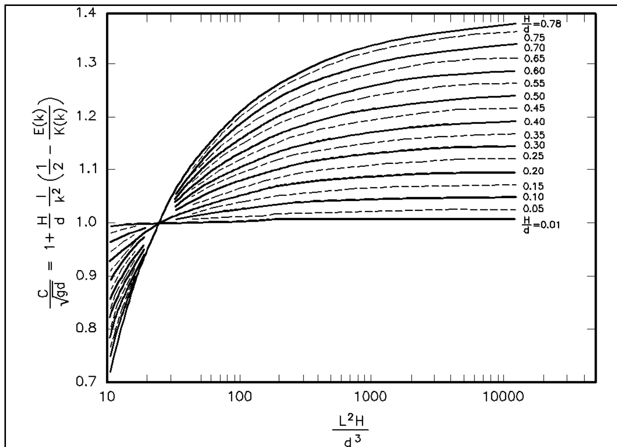
Figure II-1-16. Relationship between cnoidal wave velocity and L^2H/d^3 (Wiegel 1960)
